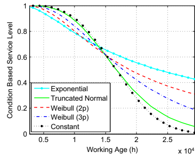
Fig. 10. CBSL for initial survival time of 3 months.
