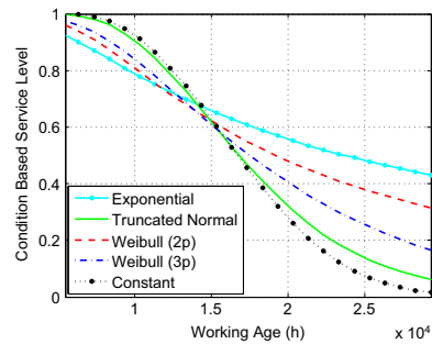
Fig. 11. CBSL for initial survival time of 6 months.
