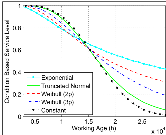
Figure 3-9: CBSL for initial survival time of 3 (months)
