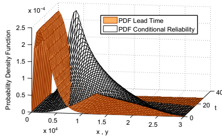
Fig. 7. Performance realization of stress versus strength.
