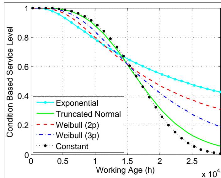
Figure 3-8: CBSL for initial survival time of 0 (months)
