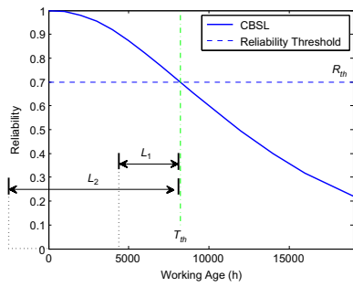
Fig. 3. Spare part ordering decision rule.
