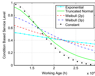
Fig. 12. CBSL for initial survival time of 12 months.
