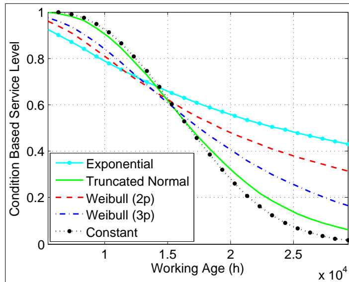
Figure 3-10: CBSL for initial survival time of 6 (months)
