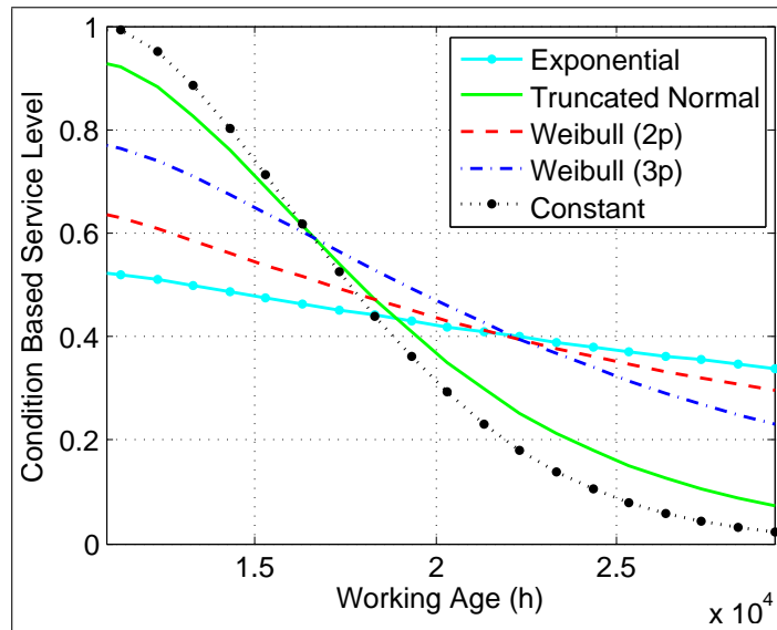
Figure 3-11: CBSL for initial survival time of 12 (months)
