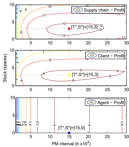
Fig. 4. Study of optimal T and S when the client subsidizes the PM cost of the agent.
