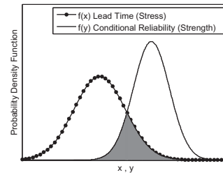
Fig. 2. CBSL as overlap of conditional reliability and lead time.
