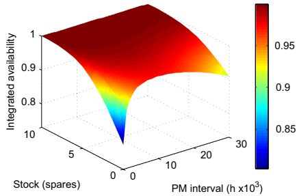
Fig. 1. System availability by integrating T and S .
