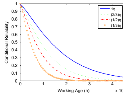
Fig. 13. Conditional reliability considering aging by depletion of \eta .
