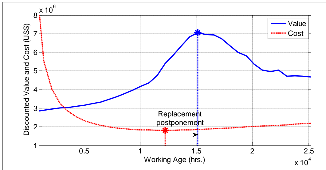
Figure 4-3: Comparison of optimal replacement times under cost and value-adding optimizations
