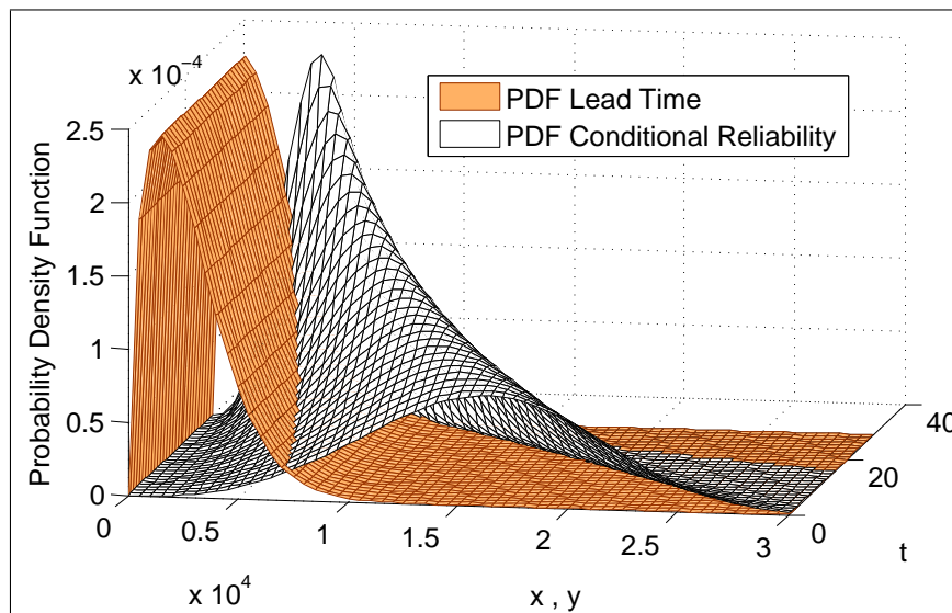
Figure 3-6: Performance realization of stress versus strength
