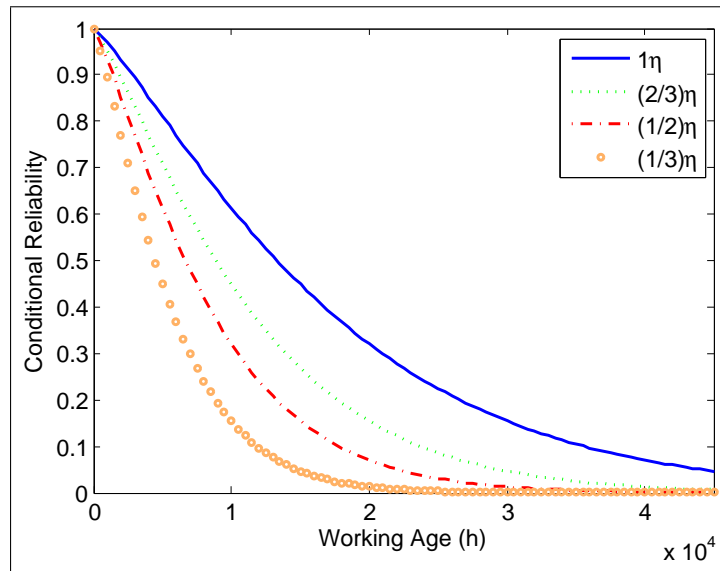
Figure 3-12: Conditional reliability considering aging by depletion of \eta
