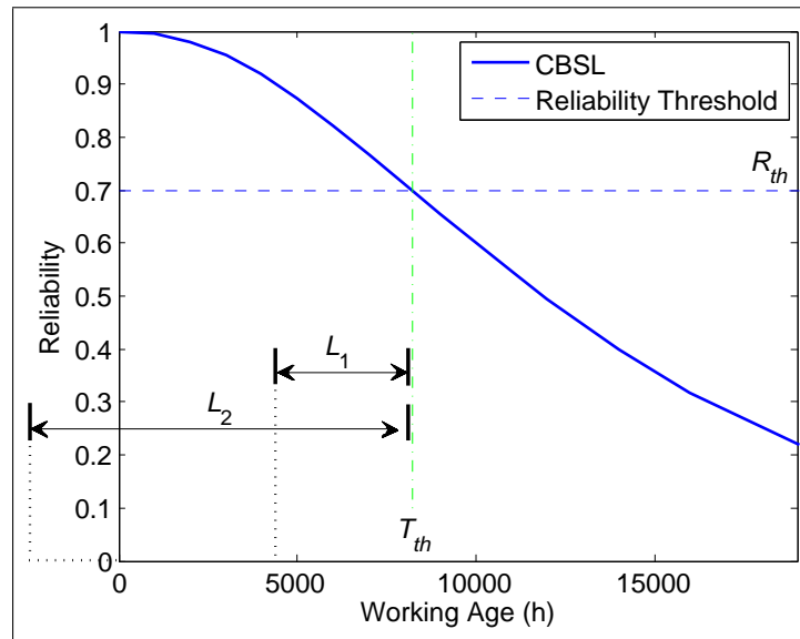
Figure 3-2: Spare part ordering decision rule
