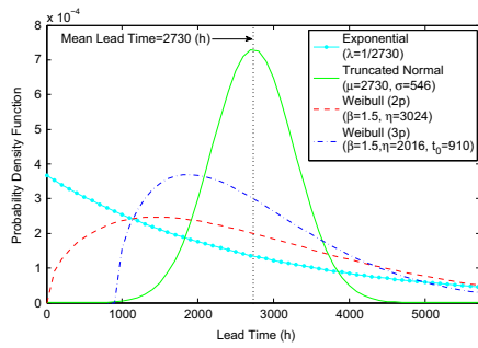
Fig. 6. Probability density functions versus lead time.
