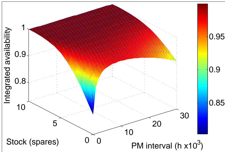
Figure 6-1: System availability by integrating T and S
