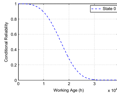
Fig. 4. Conditional reliability function at oil initial state.
