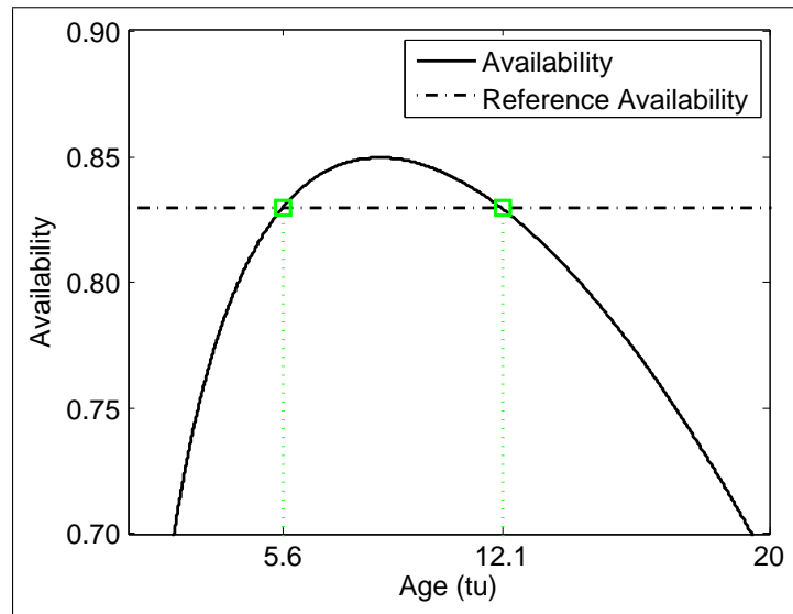
Figure 5-7: Potential solutions by setting A_r = 0.83
