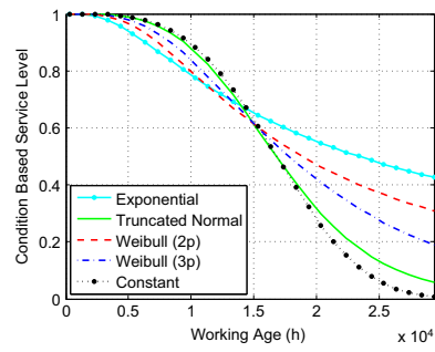
Fig. 9. CBSL for initial survival time of 0 months.
