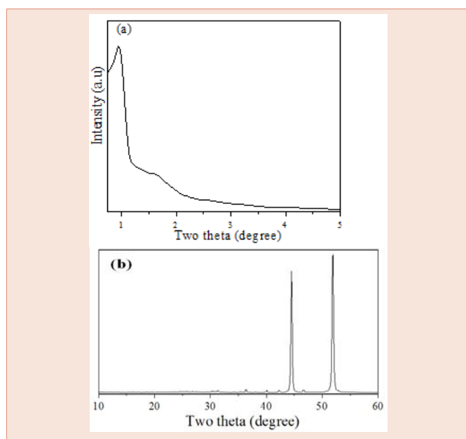
Figure 5: Fullerene mesoporous carbon (a) small angle XRD and (b) higher angle XRD patterns.
