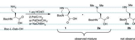
Scheme 2 Observations when performing Method D and analogous conditions.
