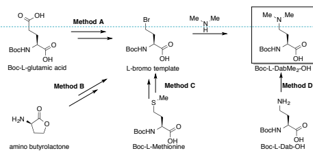
Scheme 1 Common methods found in literature. Protecting group swap from Boc to Fmoc is required as a final reaction, not shown here.
