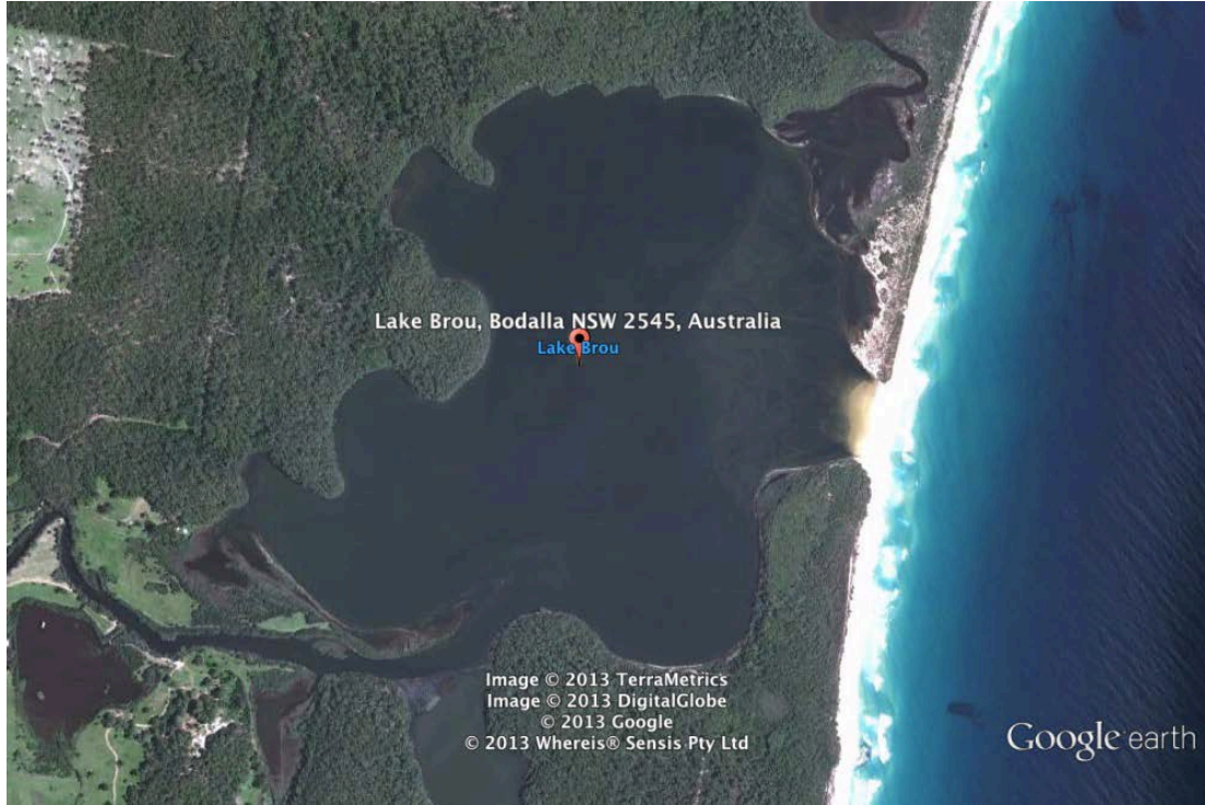
Figure 3: Lake Brou, on the South coast of New South Wales Australia ( 36^{\circ}07'S 150^{\circ}06'E ) has A_B = 2.4\text{km}^2 and faces the Tasman Sea where the mean spring tidal amplitude is around 0.5m and the mean, offshore significant wave height is approximately 1.6m corresponding to \hat{Q}_{\text{pot}} / \sqrt{gH_s^5} = 17 .
