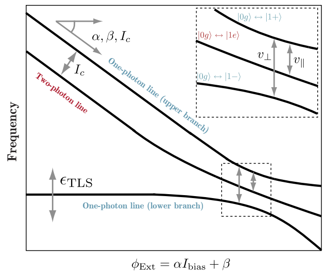
FIG. 2. (Color online) Anatomy of a qubit-TLS anticrossing in the high-power regime. The overall slope of the spectral lines, their position, and the spacing between one- and two-photon features allow us to calibrate the system, even for several independent fitting parameters (see text). The separation and asymmetry of the lines, within the anticrossing itself, allow us to estimate the transverse and longitudinal components of the coupling operator, respectively.
