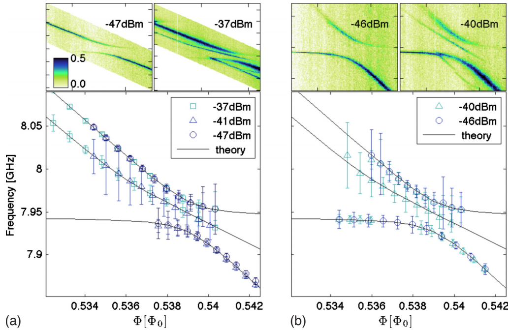
FIG. 1. (Color online) Peak positions obtained for (a) qubit spectroscopy and (b) swap-spectroscopy. For clarity, only 10% of the data set is shown. The error bars give the 1-\sigma confidence interval for the fitted peak positions. The theoretical curves show the relevant transition frequencies for the coupled qubit-TLS system obtained via fitting the extracted peak positions (see text). The inserts show examples of the (normalized) escape probability as a function of excitation frequency and bias flux, from which the peak positions are extracted.
