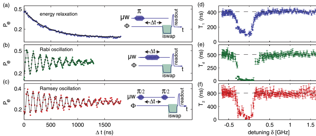
FIG. 2 (color online). Coherent response of TLS 1 to standard microwave pulse sequences as depicted in the insets. (a) Relaxation of the excited TLS state after its preparation using a microwave \pi pulse of duration 62 ns. Here, \Delta t indicates the time delay between state preparation and readout. (b) Rabi oscillation observed by driving the TLS resonantly for a duration \Delta t . (c) Ramsey oscillation measured by varying the delay \Delta t between two \pi/2 pulses (of duration 31 ns each) which were detuned from the TLS' resonance frequency by about 10 MHz. The data shown in panels (a)–(c) were obtained at a detuning \delta = 502 MHz. Panels (d), (e) and (f) show the energy relaxation time T_1^{\text{TLS1}} , the Rabi decay time T_d^{\text{TLS1}} , and the dephasing time T_2^{\text{TLS1}} as a function of the detuning \delta between TLS and qubit.
