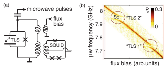
FIG. 1 (color online). (a) Schematic of the phase qubit circuit. (b) Qubit spectroscopy. Probability to measure the excited qubit state P_e after a long (300 ns) microwave pulse of small amplitude as a function of the qubit flux bias and microwave frequency. Two avoided level crossings, denoted “TLS 1” and “TLS 2”, are observed at 7.735 and 7.947 GHz with magnitudes S = 23 and 36 MHz, respectively.
