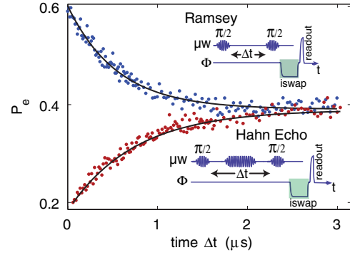
FIG. 4 (color online). Signal amplitudes obtained from Ramsey (curve starting at P_e = 0.6 ) and Hahn-echo (curve starting at P_e = 0.2 ) sequences for TLS 2. Solid lines are exponential fits resulting in a dephasing time of 551 \pm 41 ns (Ramsey) and 743 \pm 62 ns (Hahn echo), respectively.
