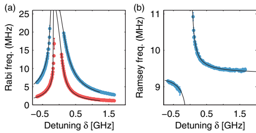
FIG. 3 (color online). (a) Rabi frequency vs detuning between TLS 1 and qubit. The two curves correspond to microwave powers differing by 9 dBm. (b) Ramsey frequency vs detuning between TLS 1 and qubit. Solid lines are calculated from theory.
