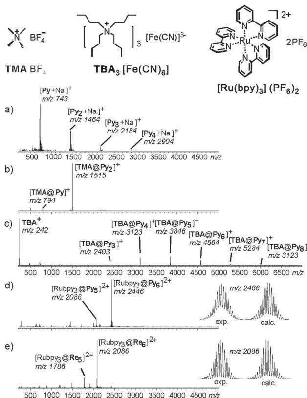
Fig. 7 Encapsulation of ionic guests by a pyrogallarene capsule is used in order to investigate the complex by ESI-FTICR. ESI-FTICR mass spectra of (a) Py , (b) after addition of TMA \text{BF}_4 , (c) TBA [\text{Fe}(\text{CN})_6]^{3-} and (d) \text{Ru}(\text{bpy})_3(\text{PF}_6)_2 . (e) Same ESI-FTICR mass spectrum recorded with Re instead of Py . Insets: experimental and calculated isotope patterns of the hexamer ions [\text{Ru}(\text{bpy})_3@\text{Py}_6]^{2+} and [\text{Ru}(\text{bpy})_3@\text{Re}_6]^{2+} . Adapted and reproduced from ref. 46 with kind permission by Wiley-VCH.
