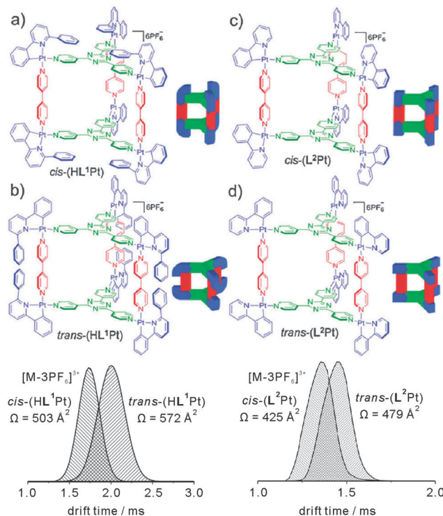
Fig. 17 Top: chemical structures of the trigonal prismatic metallo supra-molecular cages HL^1Pt and L^2Pt in their cis - and trans -forms. Bottom: IMS experiments provide sufficient resolution to distinguish both isomers by their collision cross sections. Reproduced from ref. 68 with kind permission by the Royal Society of Chemistry.
