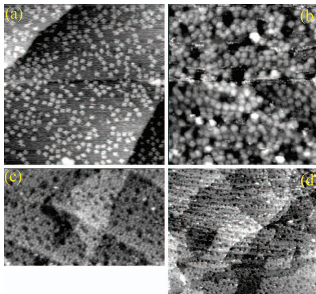
FIG. 3. Room temperature STM images of ZnPc on Pt(111); (a) Sub-ML of ZnPc/Pt(111); 360 \times 360 \text{ \AA}^2 , 60 pA, 125 mV, and multilayer of ZnPc/Pt(111): (b) 330 \times 350 \text{ \AA}^2 , 68 pA, 9 mV, (c) 900 \times 540 \text{ \AA}^2 , 68 pA, 125 mV, and (d) 1800 \times 1600 \text{ \AA}^2 , 0.8 nA, 53 mV.
