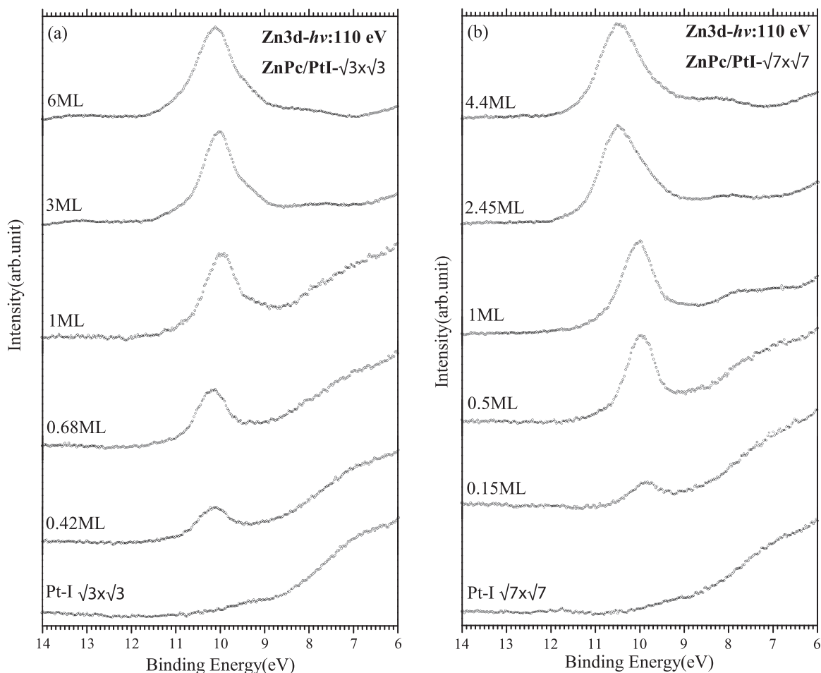
FIG. 7. Zn3d photoemission spectra of ZnPc layers on (a) Pt- (\sqrt{3} \times \sqrt{3})R30^\circ and (b) Pt- (\sqrt{7} \times \sqrt{7})R19^\circ .
