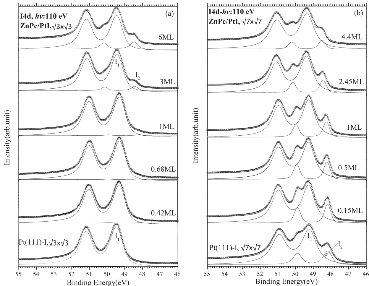
FIG. 9. I4d spectra from ZnPc on (a) PtI- (\sqrt{3} \times \sqrt{3})R30^\circ and (b) PtI- (\sqrt{7} \times \sqrt{7})R19^\circ .
