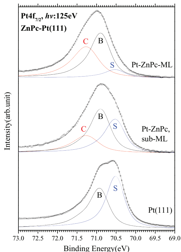
FIG. 2. Pt4f_{7/2} spectra recorded from Pt(111)-ZnPc after different preparations.
