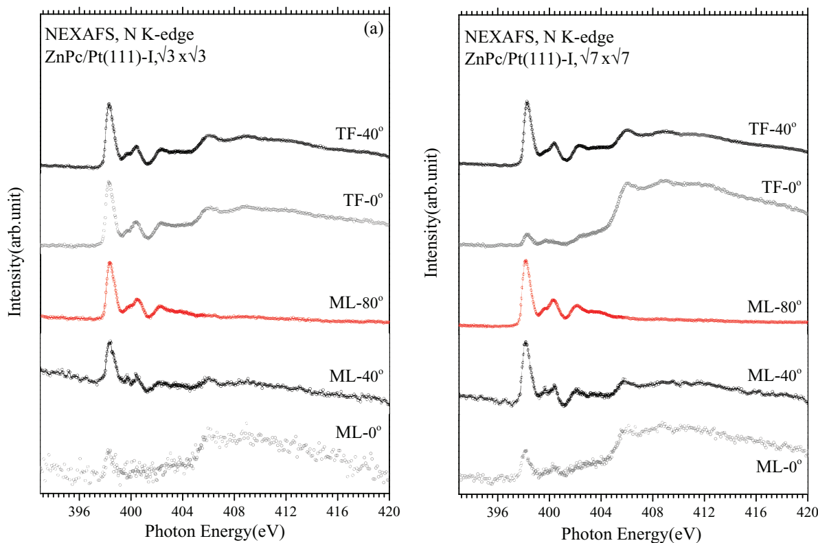
FIG. 6. N K-edge NEXAFS spectra of monolayers and thick films of ZnPc on (a) Pt- (\sqrt{3} \times \sqrt{3})R30^\circ and (b) Pt- (\sqrt{7} \times \sqrt{7})R19^\circ .
