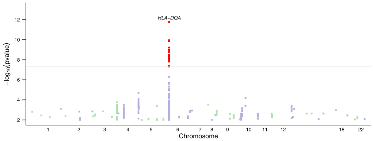
Figure 2. Manhattan plot of meta-analysis results for interactions with allergen. Results with P < 5 \times 10^{-8} are shown in red. Interaction tests were performed for markers with P < 1 \times 10^{-4} for association with at least one of cat, pollen, or dust mite allergy.
