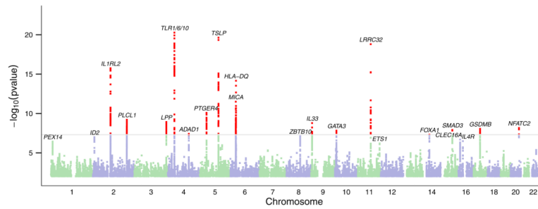
Figure 1. Manhattan plot of meta-analysis results for shared effects. The plotted values represent the most-significant scores from the meta-analyses of cat, pollen, and dust mite allergy, with all results with P < 10^{-4} recomputed using generalized estimating equations to assess effects shared across allergens. Results with P < 5 \times 10^{-8} are shown in red. Gene labels are provided for cross referencing with other results and are not intended to suggest that we have established a causal basis for the observed associations.
