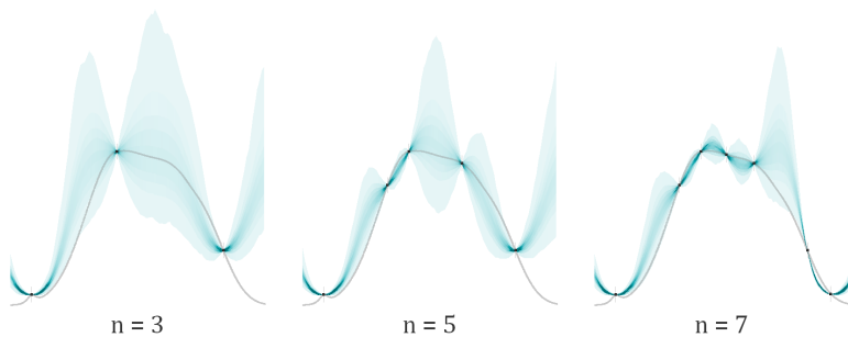
Figure 11: The target distribution (gray line) is approximated with a Gaussian process (cyan), build upon n=3, 5 and 7 points.
