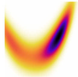
Figure 12: The heatmap of the true target distribution, used for the few next examples.
