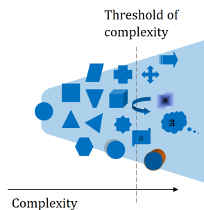
Figure 6: The set of all possible models. Should we use the simplest model possible or the most complex model which we can handle using the available computational resources?
