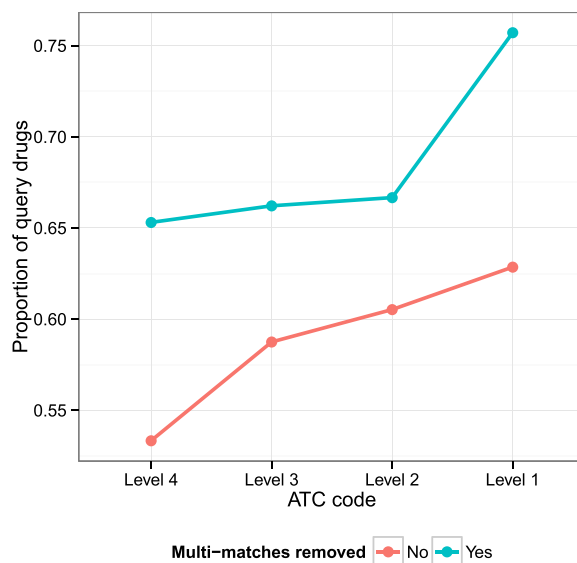
Figure 5 Combinatorial retrieval provides additional information to complement single-drug retrieval. The y-axis indicates the proportion of the query drugs for which combinatorial retrieval improves the rank for the first hit for at least one ATC code (random performance: 0.5). The results are shown for four different ATC code levels (x-axis). Red: retrieval from the full set; blue: retrieval after removing drugs having multiple ATC matches with the query.
