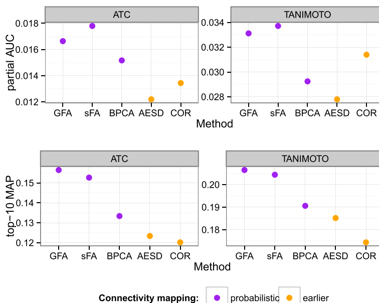
Figure 2 Probabilistic connectivity mapping outperforms earlier alternatives in retrieving similar drugs. The retrieval performance is indicated with two goodness measures (top row: partial AUC, bottom row: top-10 MAP) and two ground truths (left: ATC codes, right: Tanimoto similarity of the 2D fingerprints of the drugs). Probabilistic connectivity mapping (purple color) is performed with three models: Group Factor Analysis (GFA), sparse factor analysis (sFA), and Bayesian PCA (BPCA). These are compared to two earlier connectivity mapping methods (orange color): rank-based average enrichment-score distance (AESD) and the Pearson correlation over the differential expression profiles (COR).
