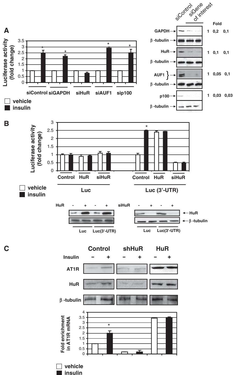
Figure 4. HuR is required for the insulin response. (A) Left panel: HEK293 cells were transfected with Luc(3'-UTR) and siRNA against either GAPDH, HuR, AUF-1, or p100 and then stimulated by 75 nM insulin for 24 h followed measurement of luciferase activity in lysates. Luciferase measurements are expressed as fold of unstimulated control. Results represent the means \pm SD of an average of three independent experiments. Lower panel: Western blots controlling the effect of gene-specific siRNA on target-protein expression and \beta -tubulin control blots. (B) HEK293 cells transfected with either Luc or Luc(3'-UTR) were transfected with either HuR or siHuR, respectively, and luciferase activity was measured in cell lysates. Results were normalized to unstimulated control transfection. Results represent the means \pm SD of an average of three independent experiments. * P < 0.05 versus unstimulated cells. Lysates were prepared and subjected to western blot analysis to monitor the expression of HuR. \beta -tubulin levels were monitored to assess the evenness of loading. (C) Coronary artery VSMC were transfected with lentiviral expression vectors of HuR and shHuR, stimulated with 75 nM insulin or vehicle for 24 h followed by western blot analysis of the protein lysates by AT1R, HuR and \beta -tubulin antibodies and qPCR analysis of mRNA. Results represent the means \pm SD of an average of three independent experiments. Right panel: qPCR of HuR in overexpression lysates or shHuR lysates.
