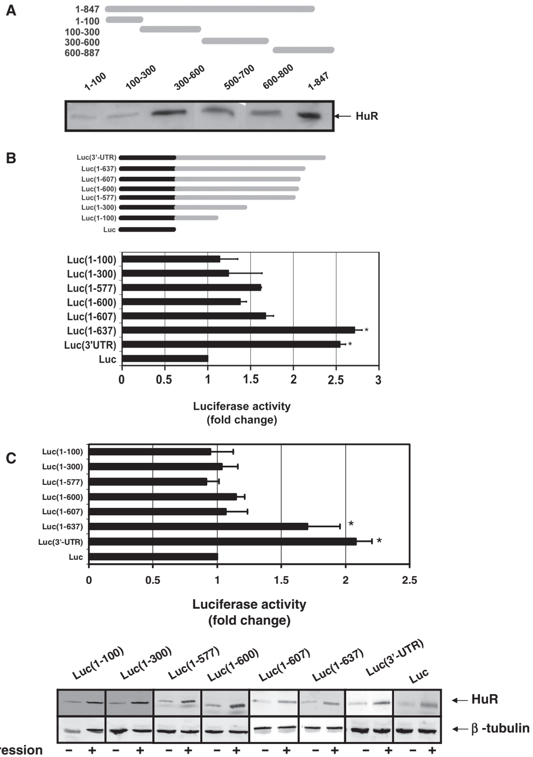
Figure 6. Insulin and HuR responsive sites are localized within the same region in the AT1R 3'-UTR (A) Upper panel: Schematic representation of the AT1R 3'-UTR mRNA fragments prepared for affinity purification. Lower panel: Mapping of the HuR binding site within AT1R 3'-UTR. RNA affinity purification was performed with different transcripts and HuR binding was measured by western blotting. (B) Mapping the insulin-responsive element within the AT1R 3'-UTR. HEK293 cells were transfected with control Luc, Luc(3'-UTR) and different deletions of 3'-UTR, treated with 75 nM insulin, and for 24h, luciferase activity was measured in the lysates. (C) Upper panel: Mapping of HuR-responsive element within the AT1R 3'-UTR. HEK293 cells were transfected with luciferase vectors as described for panel (B) and cotransfected with HuR expression vector. RNA isolated from cells described for panel (B) was subjected to real-time qPCR to assess the mRNA levels of AT1R and loading control. Results were normalized to Luc. The results represent the means \pm SD of an average of three independent experiments. * P < 0.05 versus Luc. Lower panel: Control blots for HuR overexpression.
