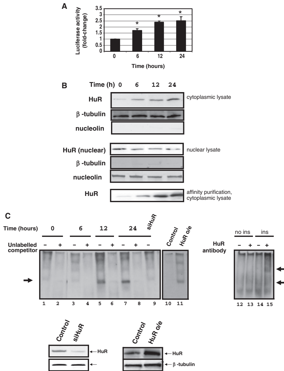
Figure 3. Increased cytoplasmic HuR after exposure to insulin. (A) At 0, 6, 12 and 24h after insulin stimulation of HEK293 cells transfected with luciferase with or without AT1R 3'-UTR, lysates were prepared to assess luciferase activity. Luminometer measurements for this experiment are expressed as fold of promoter control at time 0. The results represent the means \pm SD of an average of three independent experiments. * P < 0.05 versus without insulin stimulation. (B) Proteins isolated from cells described for panel (A) were fractionated into cytoplasmic and nuclear lysates and then subjected to western blot or to affinity purification using AT1R 3'-UTR as probe. \beta -tubulin and nucleolin were detected in the lysates to monitor for the purity of the fractionation. Data representative of three independent experiments is shown. (C) To demonstrate an increased binding of HuR to AT1R 3'-UTR in response to insulin, EMSA assays were performed using lysates from cells described in panel (A). Cytoplasmic lysates were assayed in EMSA with labeled RNA probe corresponding to nucleotides 1–847 of AT1R 3'-UTR. After binding, the samples were RNAase treated to reduce background due to non-specific binding. Lanes 1–8 show a time course of insulin effect on HuR binding to AT1R 3'-UTR. Lanes 2, 4, 6 and 8 were treated with a 10-fold excess of unlabeled 1–847 probe. The cells used to prepare lysates for a gel shift shown in Lanes 1–8 were untransfected, whereas in Lane 9 cells were transfected with siHuR. In Lanes 10 and 11, same probe 1–847 was used but either with control (10) or HuR overexpression lysates were used (11). In insulin-stimulated cells (lanes 14,15) incubation of the cytoplasmic lysates with HuR-specific antibody caused a gel shift (lane 15). The western below blots document the effect of HuR silencing and overexpression by densitometry.
