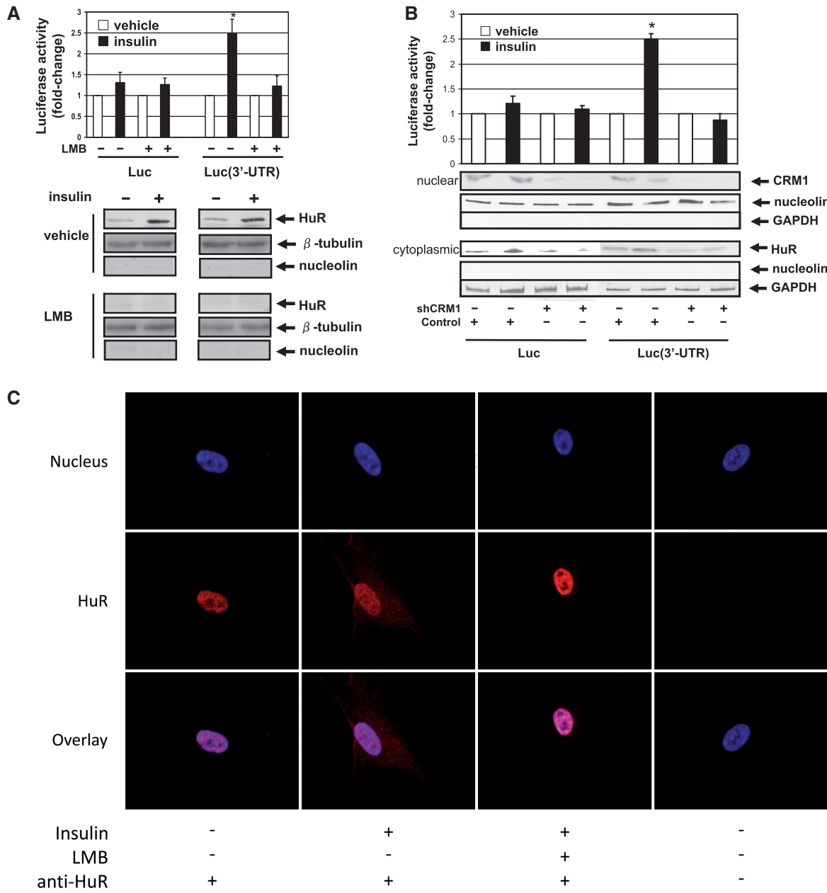
Figure 7. Translocation of HuR mediates insulin effect on AT1R. (A) Upper panel: HEK293 cells transfected with Luc or Luc(3'-UTR) were stimulated with insulin in the presence or absence of LMB for 12 h and lysates were measured for luciferase activity. Luciferase results are expressed as fold of promoter control without 3'-UTR in relative light units of firefly luciferase. Results represent the means \pm SD of an average of three independent experiments. Lower panel: Protein lysates from cells described for panel (A) were extracted and probed for the expression of HuR, nucleolin and \beta -tubulin. (B) Upper panel: HEK293 cells transfected with Luc or Luc(3'-UTR) and cotransfected with either shCRM1 or shControl. Insulin stimulation (75 nM) for 24 h followed by determination of luciferase activity on the cell lysates. Luciferase results are expressed as fold of promoter control without 3'-UTR in relative light units of firefly luciferase. Results represent the means \pm SD of an average of three independent experiments. Lower panel: Protein lysates from cells described for panel (B) were extracted and probed for the expression of CRM1, HuR, nucleolin and GAPDH. (C) Immunofluorescence analysis of HuR. HuR signals (red) in either untreated or insulin treated (75 nM for 12 h) coronary artery VSMC cells. Red, HuR fluorescence; blue, DAPI staining to visualize nuclei; overlay, overlap of the two signals. Note the distinct overlap of DAPI and HuR signals in untreated cells; while insulin-stimulated cells also exhibit abundant nuclear HuR, the treatment causes a substantial increase in the cytoplasmic HuR signal, not seen in untreated cells. Exposure to LMB prevented the insulin effect.
