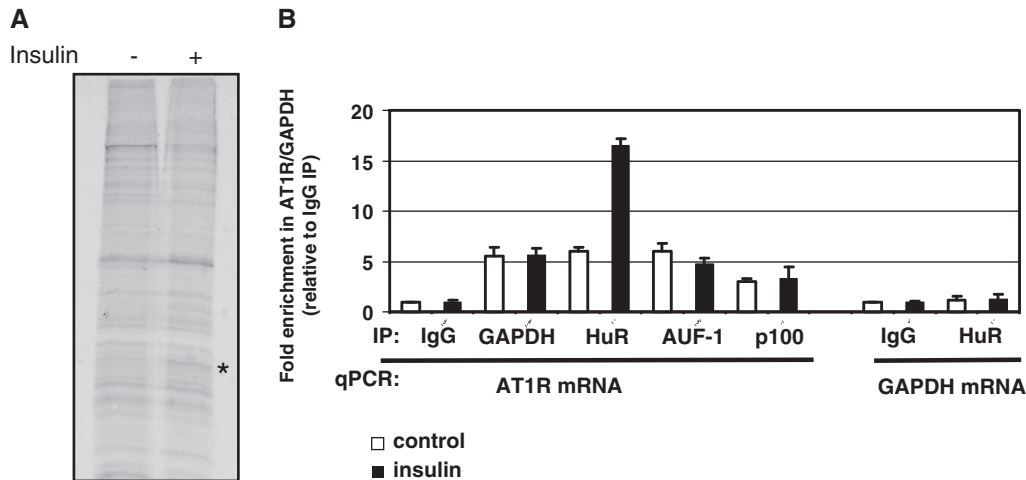
Figure 2. Insulin increases the interaction of HuR with AT1R 3'-UTR. (A) Twenty-four hours after insulin or vehicle stimulation of coronary artery VSMCs, lysates were prepared to affinity purify proteins by using AT1R 3'-UTR mRNA as a bait. A silver stained SDS-PAGE gel shows a differential expression of a 36-kDa protein (asterisk) which was then excised, digested and recognized by mass spectrometry. The details of the purification are given under "Experimental procedures". (B) Proteins isolated from cells described for panel (A) was subjected to IP by HuR-, GAPDH-, AUF1-, p100, or as a control preimmuno IgG antibodies followed by RNA extraction and qPCR of either AT1R or GAPDH as a control. Results represent the means \pm SD of an average of three independent experiments performed as a triplicate for each construct. * P < 0.05 versus control stimulation.
