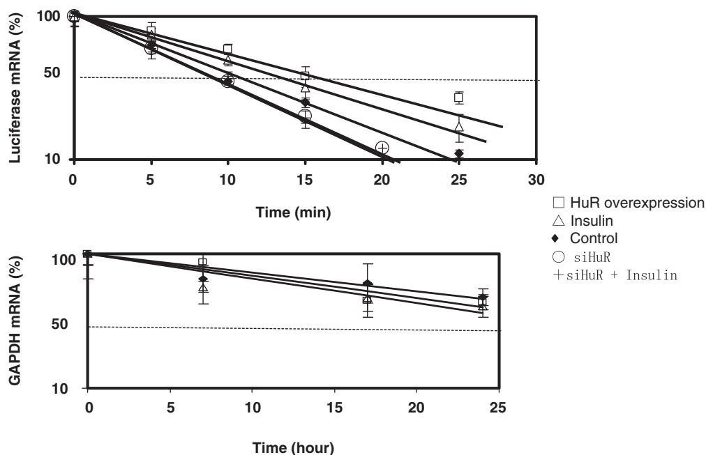
Figure 5. The ectopic modulation of HuR expression alters the insulin effect on AT1R 3'-UTR half-life. HEK293 transfected with Luc(3'-UTR) had their cytoplasmic HuR levels altered by cotransfection of either HuR expression vector or siHuR or stimulation by insulin. Cells were exposed to actinomycin D (2 \mu g/ml), whereupon the cellular RNA was isolated at the times indicated and subjected to real-time qPCR to assess the half-life of Luc mRNA. In the upper panel, luciferase qPCR. Lower panel: GAPDH qPCR. Results represent Luc or GAPDH mRNA normalized to the expression of the construct at time 0. Results are shown as a linear fit. Results represent the means \pm SD of an average of three independent experiments.
