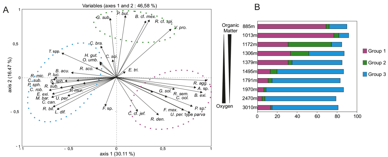
Fig. 6. (a) PCA plot based on the relative abundances of the dominant species (> 2 % in at least one station) for the entire core (0–10 cm) in the > 125 μm size fraction. (b) Plot of the percentages of the three defined groups at the various sites.
