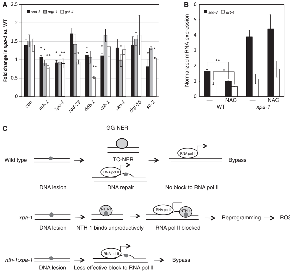
Figure 5. NTH-1 and XPC-1 are upstream factors required for transcriptome modulation in xpa-1 . (A) Transcript levels of sod-3 , aqp-1 and gst-4 were measured by qRT-PCR in WT or xpa-1 nematodes fed with RNAi constructs targeting nth-1 , xpc-1 , rad-23 , ddb-1 , csb-1 , skn-1 and daf-16 . All transcript levels were normalized to that of gamma-tubulin ( tbg-1 ) and presented as fold-changes relative to the WT. (B) Transcript levels measured in WT or xpa-1 mutants in the absence (-) or presence of the antioxidant NAC. (C) Cartoon showing the working model: in the WT situation (top), transcription-blocking lesions (small circle) do not accumulate and are not processed by BER. In the absence of xpa-1 (middle) the NER pathway is not functioning, leaving NTH-1 to bind unprocessed DNA lesions. This generates genomic stress signals and activates reprogramming, which induces ROS generation. When both xpa-1 and nth-1 are missing (bottom) there is no DNA repair enzyme that may bind the lesion site, the lesion is bypassed and no reprogramming is initiated. The results are presented as average \pm SEM from at least three independent replicates. * P < 0.05 , ** P < 0.01 ; Student's t -test.
