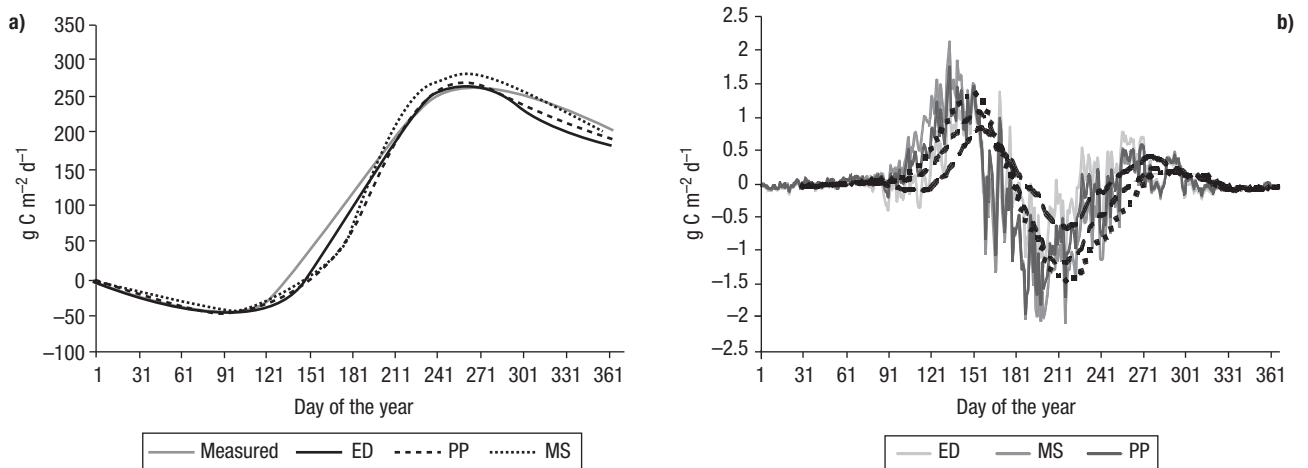
Figure 6. a) Measured and simulated cumulative net ecosystem exchange (positive numbers indicate a gain in biosphere carbon). Each data point is the average of ten simulated values throughout the period from 1998 to 2007. b) Differences between measured and simulated net ecosystem exchange rates. The black lines refer to smoothed 30 day averages of simulations obtained with different stand structural assumptions (same line structure as in figure above).
