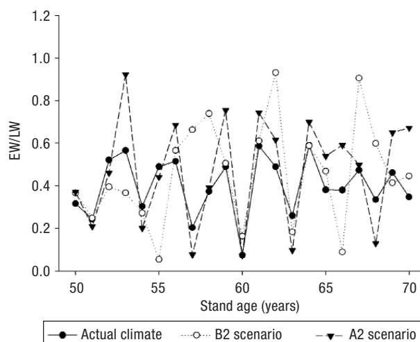
Figure 9. Simulated EW/LW ratio under three climate scenarios: actual climate, moderate (B2) and severe (A2) climate change.
