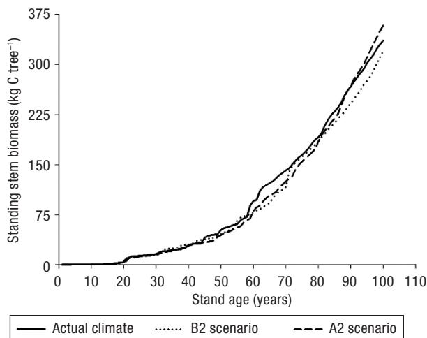
Figure 8. Simulated standing biomass development of pedunculate oak under three climate scenarios: actual climate, moderate (B2) and severe (A2) climate change.
