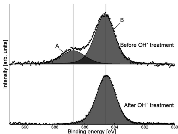
Fig. 8 High-resolution F XPS signal for \text{NH}_4\text{PF}_6 -modified \text{TiO}_2 , before and after washing with KOH.
