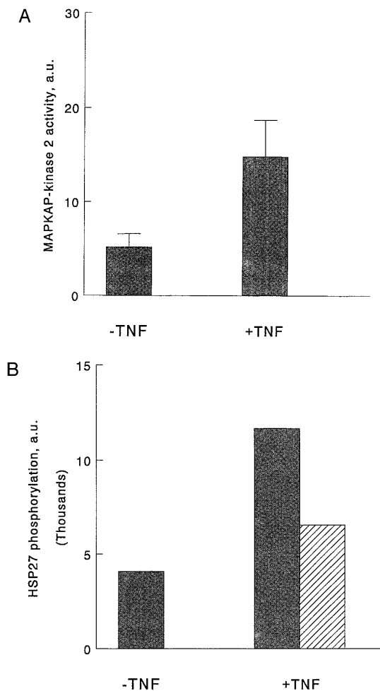
FIG. 1. Activation of MAPKAP kinase 2 activity in endothelial cells stimulated with 100 U/ml \text{TNF}\alpha . After 10 min of stimulation cells were lysed, and MAPKAP kinase 2 was immuno-precipitated. Enzymatic activity was assessed by Hsp25 phosphorylation in vitro . Data are presented as mean \pm sem, n=3 . (b) \text{TNF}\alpha stimulated Hsp27 phosphorylation in endothelial cells. ^{32}\text{PO}_4^{3-} pre-loaded cells were treated with or without 100 U/ml \text{TNF}\alpha for 10 min, in the absence (grey bars) or presence (hatched bars) of 20 \mu\text{M} SB203580. Hsp27 was immuno-precipitated and subjected to SDS-PAGE. Radioactivity in the Hsp27 band was quantitated by phospho-imaging. The results are representative of two independent experiments.
