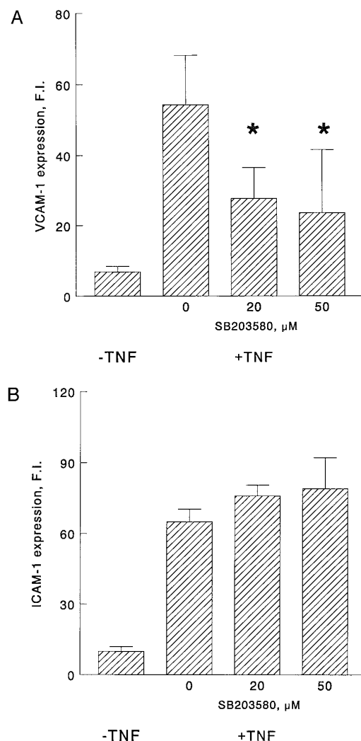
FIG. 2. Effect of SB203580 on the \text{TNF}\alpha -induced expression of VCAM-1 (a) and ICAM-1 (b). Confluent monolayers of endothelial cells were pretreated with 20 or 50 \mu\text{M} SB203580 for 30 min, and subsequently stimulated with 100 U/ml \text{TNF}\alpha for 6 h also in the presence of SB203580. The expression of VCAM-1 and ICAM-1 was assessed by FACS analysis. The results are expressed as fluorescence intensities (mean \pm sem, n=3-5 ). Asterisks indicate a significant difference from the untreated control. (Student's t-test, p<0.05 ).
