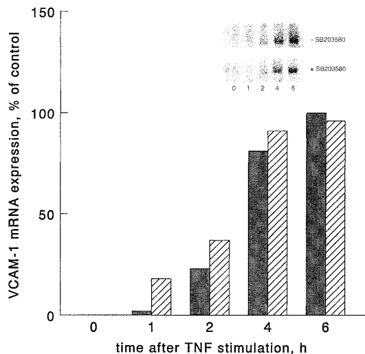
FIG. 3. Time course of the TNF \alpha -induced expression of VCAM-1 mRNA. After 30 min pretreatment with 20 \mu M SB203580 or vehicle endothelial cells were stimulated with 100 U/ml TNF \alpha in the presence (hatched bars) or absence (grey bars) of SB203580. Total RNA was isolated and size-fractionated by denaturing 1.2% agarose-formaldehyde gel electrophoresis, transferred to nitrocellulose, and hybridized to ^{32} P-labeled human VCAM-1-specific cDNA (inset). Data are representative of three independent experiments.
