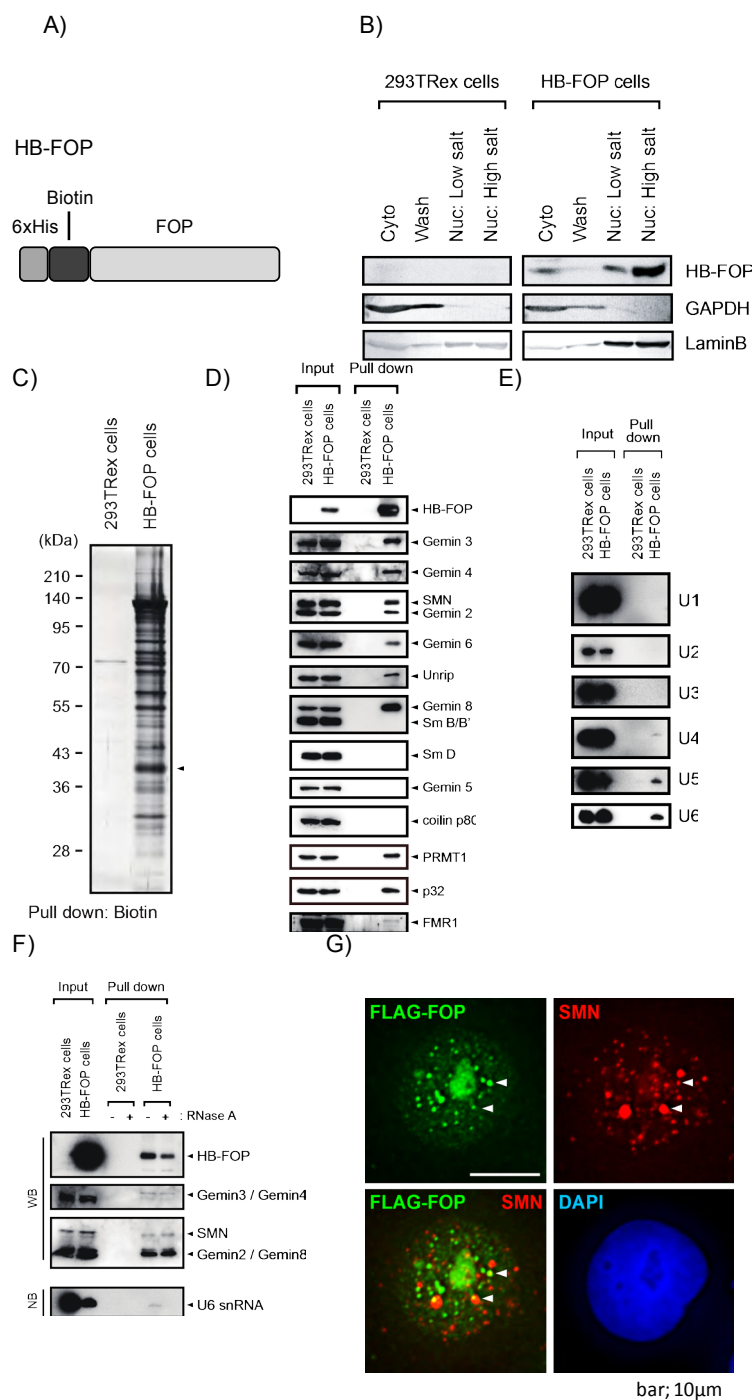
Figure 3: FOP-associated nuclear SMN complex lacks Gemin5 and coilin as well as U1 and U2 snRNAs. (A) Schematic representation of FOP tagged with DAP lacking FLAG (HB-FOP). (B) 293TRex cells stably expressing HB-FOP (HB-FOP cells) were fractionated into cytoplasmic extract (Cyto), cytoplasm wash fraction (Wash), and nuclear extract at low salt condition (Nuc: Low salt) or at high salt condition (Nuc: high salt) (see Material and methods). They were analyzed by western blot method with the antibodies against Lamin B and GAPDH, respectively. HB-FOP was detected with HRP-conjugated streptavidin. Parental 293TRex cells were used as a control (293TRex cells). (C) HB-FOP complex was pulled down from the nuclear extract of HB-FOP cells or 293TRex cells with avidin-fixed beads (Biotin), separated by SDS-PAGE and visualized by silver staining. The protein band of HB-FOP was assigned based on its mobility expected from the amino acid sequence of HB-FOP on SDS-PAGE gel. Molecular weights of the marker proteins are indicated at left. (D) The pulled-down HB-FOP complex were analyzed by western blot with the antibodies indicated at the right. HB-FOP was detected with HRP-conjugated streptavidin. Total RNA (1 μg) was used as input. (E) The RNAs extracted from the HB-FOP complex were analyzed by northern blot with the biotin labeled DNA probes complementary to U1-U6 sn(0)RNAs, respectively. (F) The pulled-down HB-FOP complex was analyzed by western blotting with the antibodies against proteins indicated at the right with (+) or without (-) RNase A treatment. U6 snRNA was detected by northern blot analysis. (G) 293TRex cells inducibly expressing FLAG-fused-FOP (FLAG-FOP cells) were subjected to immunocytochemical analysis with the antibody against FLAG (green) or endogenous SMN (red) after the removal of the cytoplasmic proteins by permeabilization with Triton. DAPI staining (blue) shows the nucleus. Scale bar: 10 μm.
