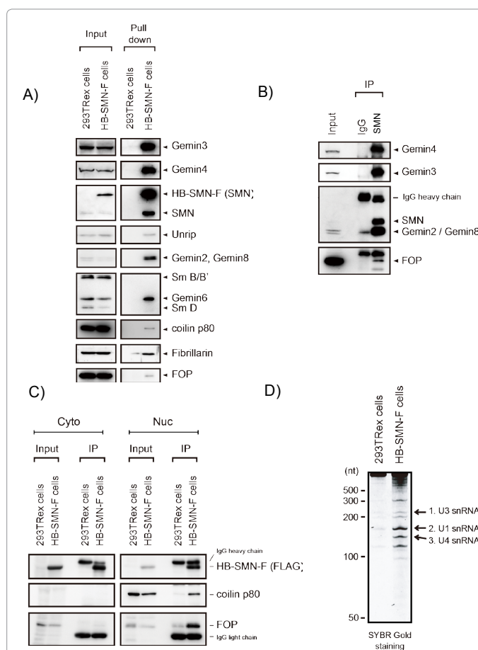
Figure 2: The nuclear SMN complexes isolated contain FOP but not SmB/B' and SmD. (A) The nuclear SMN complexes were pulled down from the nuclear extract of parental 293TRex cells or from 293TRex cells expressing HB-SMN-F (HB-SMN-F cells) by biotin affinity method, and analyzed by western blotting with the antibodies indicated at the right. (B) Endogenous SMN complexes were immunoprecipitated from the nuclear extract of 293TRex cells with anti-SMN antibody or control IgG(IgG), and analyzed by western blotting with the antibodies indicated at the right. A staining band corresponding to that of IgG heavy chain is also indicated. (C) SMN complexes were immunoprecipitated with anti-FLAG M2 antibody fixed beads from cytoplasmic or nuclear extract of HB-SMN-F or parental 293TRex cells, and analyzed by western blotting with the antibodies indicated at the right. A staining band corresponding to that of IgG light chain is also indicated. (D) RNAs extracted from the SMN complexes isolated from the nuclear extract of HB-SMN-F cells or 293TRex cells were separated by denaturing urea PAGE and stained with SYBR gold. The RNAs in the staining bands (1-3) are identified by LC-MS/MS-Ariadne analysis, and the identified RNAs are indicated at the right.
