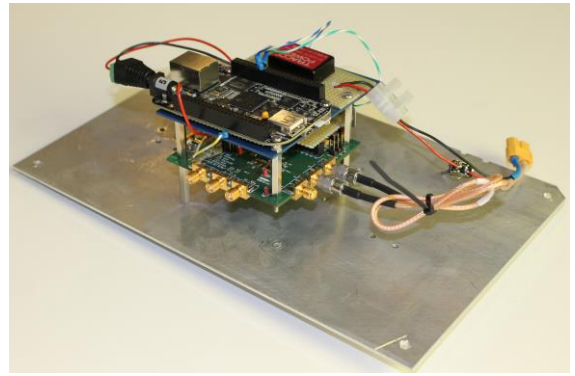
Figure 6: GNSS sampler mounted on 20 x 25 cm aluminium-plate (UAV payload). The MAX2769 EV-KIT is the bottom circuit with the BeagleBone Black and a power-supply board fitted on top.
