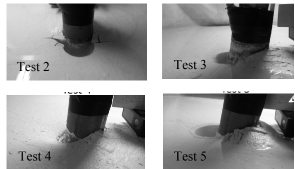
Figure 5. Failure mode after lateral loading for the 4 tests.
