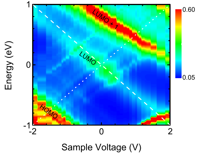
Figure 5. Density plot of the transmission function, T(E, V) = \sum_n \tau_n(E, V) , for different energies E and voltages V in the contact range. The energies of the transmission maxima labelled HOMO, LUMO, and LUMO+1 approximately follow the chemical potential of the sample -eV/2 (dashed line). Weaker transmission features are related to tip states and follow the chemical potential of the tip +eV/2 , (dotted line).
