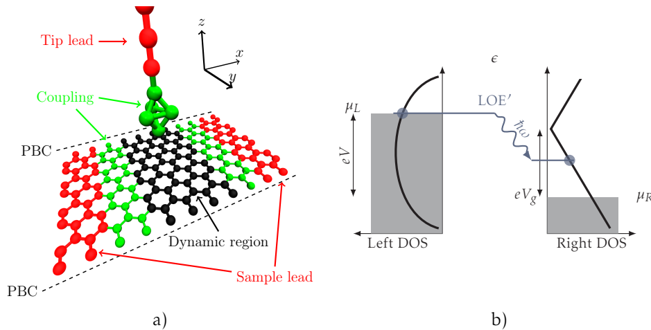
Figure 8.3 | a) Method setup for calculating the first-principle study of inelastic tunnelling into graphene. Phonon region (black atoms), electron-phonon coupling region (black+green), electrodes (red). From [171]. b) At and above threshold, eV = \hbar\omega , LOE adds a constant inelastic contribution for said phonon. While the LOE' constantly follows the chemical potential of the left and estimates the contribution at threshold for all phonons thus probing the Right DOS.
