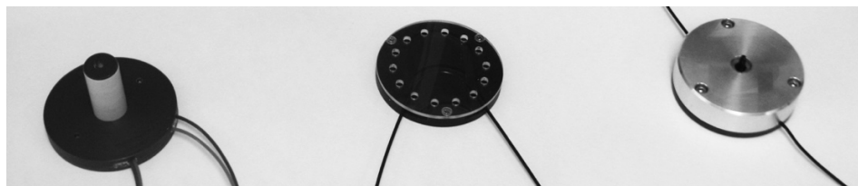
Figure 1: standard flow cell (left); capillary holder (middle); self-build lead insert (right)
