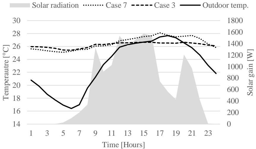
Figure 5 – Temperatures during a hot summer day
