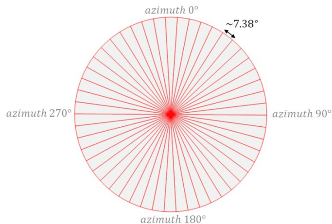
Figure 3. Scanning geometry of the ZDM lidar: \sim 50 LOS / revolution
