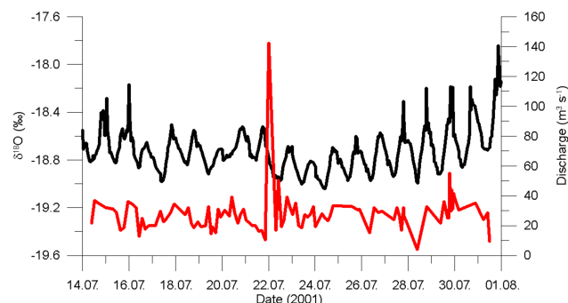
Figure 4. Time series of \delta^{18}\text{O} (red curve) and discharge (black curve) in the Kuannersuit Glacier river during the period 14–31 July 2001.
