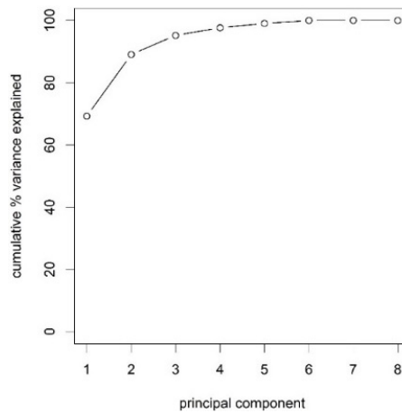
Figure 2. Cumulative % of the variance in the dataset captured by the first 8 principal components.
