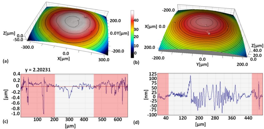
Fig. 8. Topography image with height contours for each 2 \mu\text{m} in the z-direction for micro-lenslet from (a) (shown 600 x 600 \mu\text{m}^2 area) uncoated and (b) (shown 400 x 400 \mu\text{m}^2 area) coated mold and corresponding surface variation along cross section in (c) and (d) respectively.
