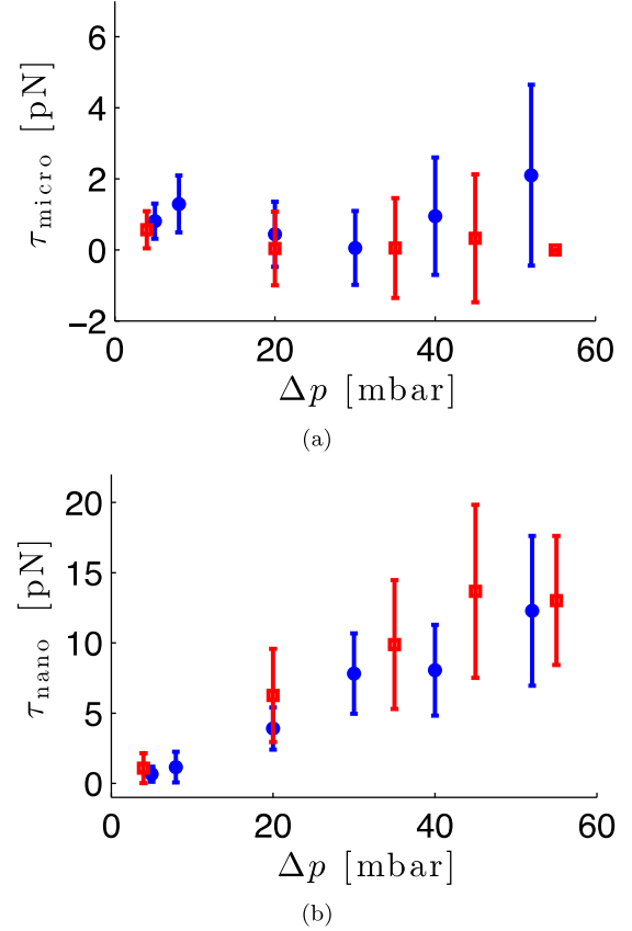
FIG. 5. Fits of \tau_{\text{micro}} [panel (a)] and \tau_{\text{nano}} [panel (b)] for common values of \sigma_{\text{pos}} and \gamma^\perp for two different DNA molecules. \Delta p is the pressure drop, see Fig. 1(a). Error bars are simulated standard deviations of the fitted parameters.
