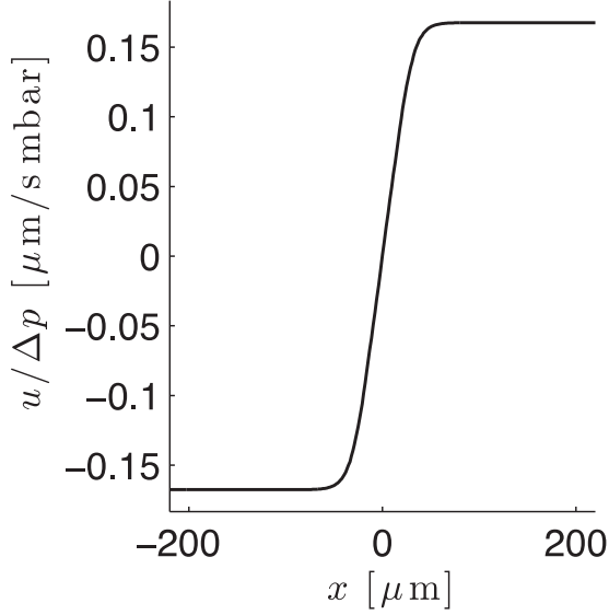
FIG. 3. Flow velocity averaged along the z direction u over the pressure drop along the x axis calculated with COMSOL MULTIPHYSICS for the geometry shown in Fig. 1. The Navier-Stokes equation [Eq. (C1)] is solved under the “Shallow Channel Approximation”.
