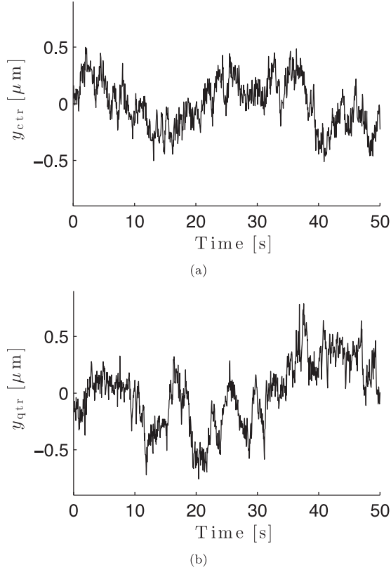
FIG. 2. The transverse motion of the DNA at the points x_{ctr} [panel (a)] and x_{qtr} [panel (b)] for an applied pressure \Delta p = 40 mbar.
