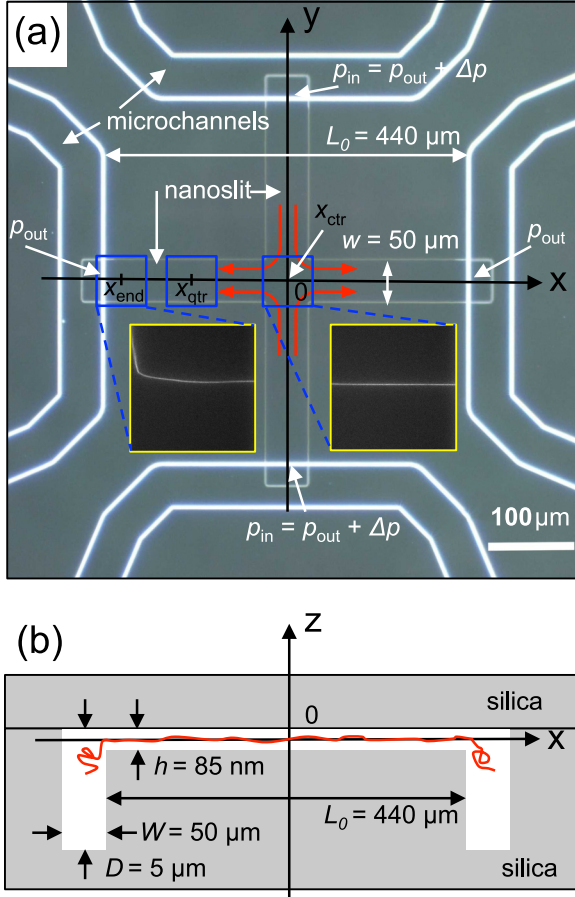
FIG. 1. (a) SEM image of the chip showing a cross-shaped nanoslit connected to four microchannels. A pressure difference \Delta p is applied between the microchannels intersecting the y axis and the microchannels intersecting the x axis. This causes a flow indicated by the red arrows with a stagnation point at the center of the chip. Blue boxes mark the three fields of view used in the analysis of the motion of the DNA. Yellow-edged insets show images of a DNA molecule stretched by the flows. Notice the kink in the DNA at the interface between the nanoslit and the microchannels. (b) Schematics of the cross section of the chip along the x axis (not to scale). The nanoslit is 440 \mu\text{m} long and 50 \mu\text{m} wide but only 85 \text{ nm} high. The microchannels are 5 \mu\text{m} deep and 50 \mu\text{m} wide. A DNA molecule, stretched between the microchannels, is sketched in red.
