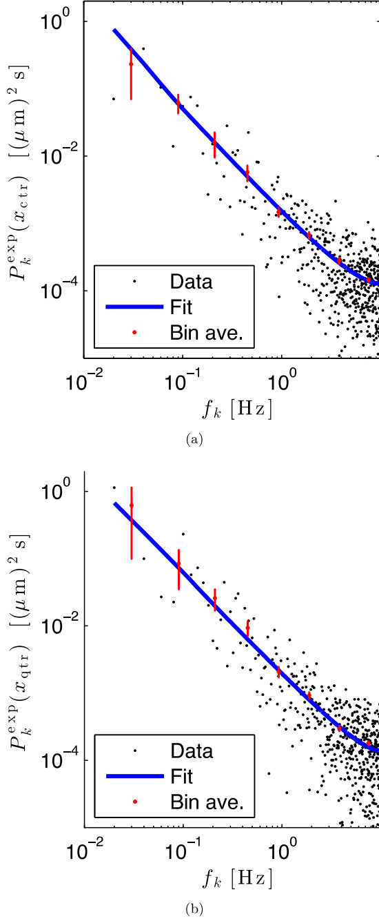
FIG. 6. Panels (a) and (b) show the power spectra for the time series of the positions recorded at x_{\text{ctr}} and x_{\text{qtr}} , respectively, for a pressure drop \Delta p = 40 mbar. Black dots are the experimental power spectral values P_k^{\text{exp}}(s) [Eq. (19)]. Red dots are bin averages with error bars indicating standard errors on the means. Blue lines are fits to Eq. (24) with the constraint that \tau_{\text{nano}} = a\Delta p and common values for the transverse friction coefficient \gamma^\perp and the localization error \sigma_{\text{pos}} (see Sec. VIII for details). P values for Pearson's \chi^2 goodness-of-fit test are 0.77 and 0.23, respectively.
