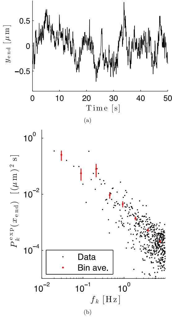
FIG. 8. Panel (a) shows the transverse motion of the DNA at the position x_{\text{end}} located 20 \mu\text{m} from the microchannel for the same DNA molecule as in Fig. 2 and a pressure drop of \Delta p = 40 \text{ mbar} . Panel (b) shows the corresponding power spectral values. Error bars are standard errors on the means.
