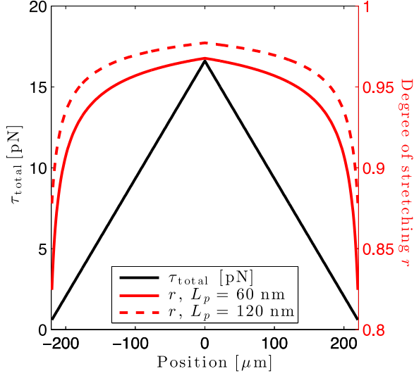
FIG. 4. Black curve, left axis: Total tension \tau_{\text{total}} in the DNA versus the position in the nanoslit from Eq. (3) using the parameters for the tensions \tau_{\text{micro}} = 0.6 pN and \tau_{\text{nano}} = 16 pN. The length of the nanoslit is L_0 = 440 \mu\text{m} . Red curves, right axis: Corresponding degrees of stretching r calculated with Eq. (26) for the two different values of the persistence length L_p discussed in the main text.
