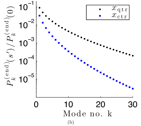
FIG. 9. Upper bounds for the ratios of the power spectra P_k^{(\text{end})}(s')/P_k^{(\text{end})}(0) . Input parameters are \tau_{\text{nano}} = 15 pN, \tau_{\text{micro}} = 0.6 pN, \gamma^\perp = 1.9 \times 10^{-3} pN s/ (\mu\text{m})^2 , and L_0 = 440 \mu\text{m} . Panel (a) shows the ratio versus position s' for the longest propagating mode, i.e., the mode with k = 1 . The black curve is the exact expression [Eq. (D14)], while the red and the blue curves are the approximations in Eqs. (D16) and (D17), respectively. Panel (b) shows the exact ratio at the two positions s' = x_{\text{qtr}} and s' = x_{\text{ctr}} used in the analysis of the tension versus the mode number k .
