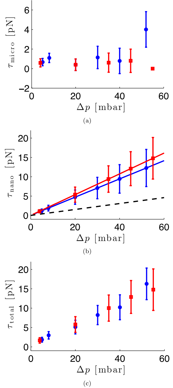
FIG. 7. Fits for common values of \sigma_{\text{pos}} and \gamma^\perp with the constraint that \tau_{\text{nano}} = a \times \Delta p for two different DNA molecules ( \Delta p is the pressure drop). Panel (a) shows \tau_{\text{micro}} , panel (b) \tau_{\text{nano}} , and panel (c) the total tension at the center of the nanoslit, i.e., \tau_{\text{total}} = \tau_{\text{micro}} + \tau_{\text{nano}} . The dashed line in panel (b) marks the tension induced by the estimated drag force on a cylinder with a radius R_H = 1 nm placed at the center of the slit (see Sec. IX). Error bars are simulated standard deviations of the fitted parameters.
