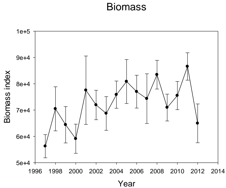
Fig. 2. Biomass (tons) of Greenland halibut in Div. 1CD by year with 1 * \text{S.E.} . No data from 2013.
