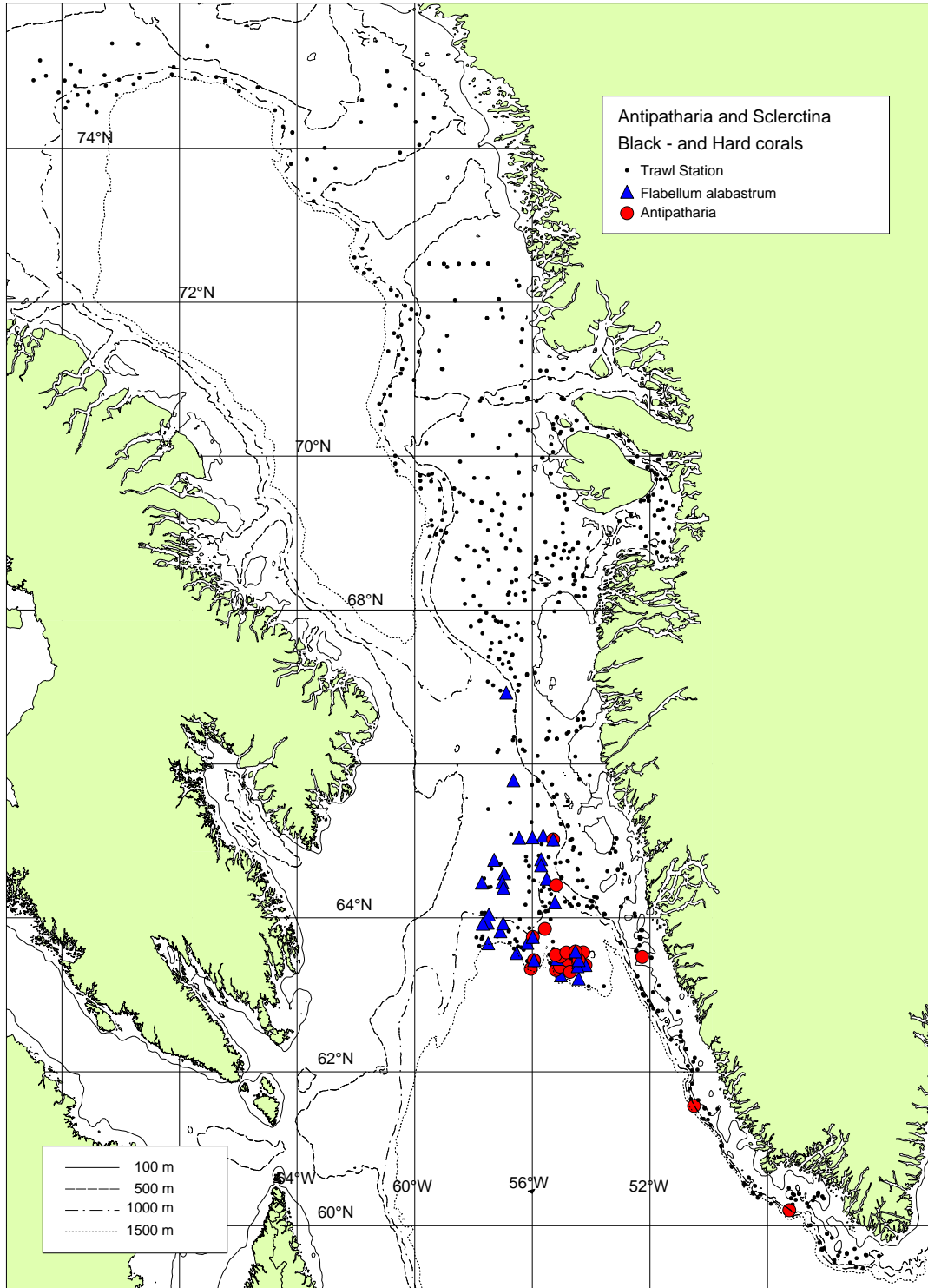
Fig. 4. Distribution of black and stony corals (Antipatharia and Sclerctinia).
