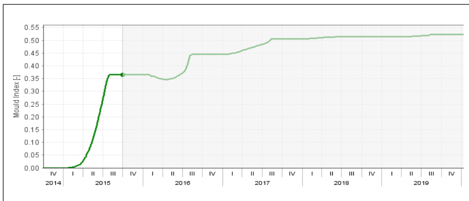
12 13 Figure 12. Mould index for impregnated original wall + IQ-Therm 50 mm + façade crack 1 cm deep 14
