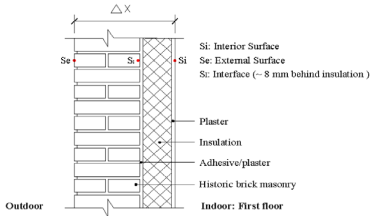
2 Figure 1. Principle drawing of investigated masonry wall with insulation and location, where the simulated output is used for 3 analysis (S i : Interior surface, S e : External surface (outside) and S i : Interface between original wall and insulation)
