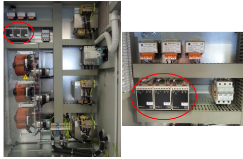
Fig. 10. Control Unit
