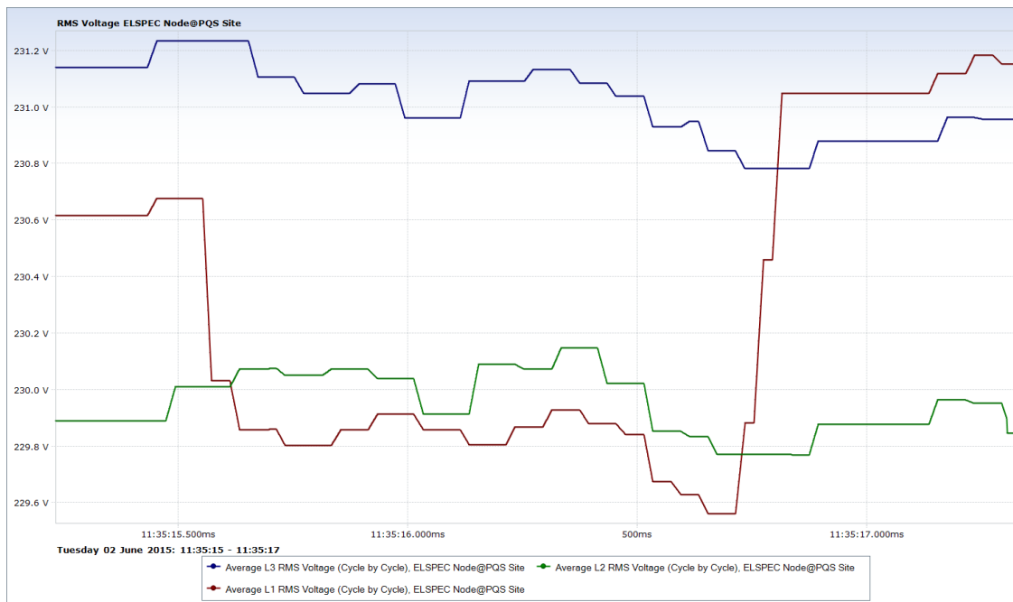
Fig. 23. 11:35 – Event #2: zoom-in of the phase-neutral voltage on phase a
