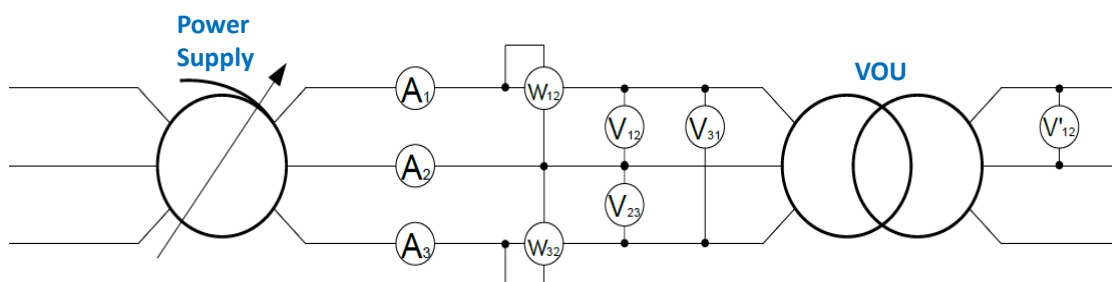
Fig. 36. Circuit diagram for open circuit test
