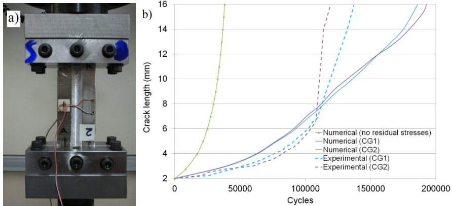
Fig. 3 a) Experimental setup for crack propagation test. b) Comparison between numerical and experimental crack advances vs. number of cycles.
