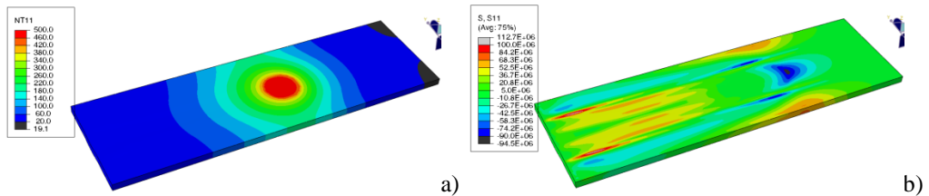
Fig. 2 a) Temperature field from the heat transfer analysis after 100 s of welding. b) The resulting longitudinal stress component from the stress analysis at the same time step.
