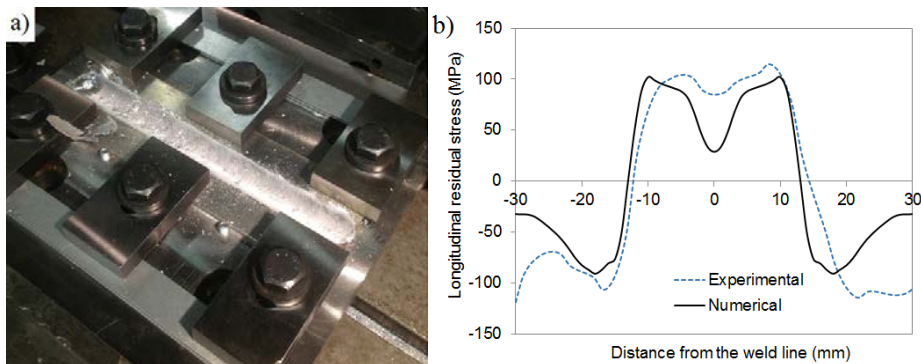
Fig. 1 a) Welding setup. b) Comparison of longitudinal residual stresses from experiment and simulation.
