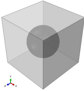
Figure 1: Micromechanical periodic unit cell representing the microstructure of DCI.
