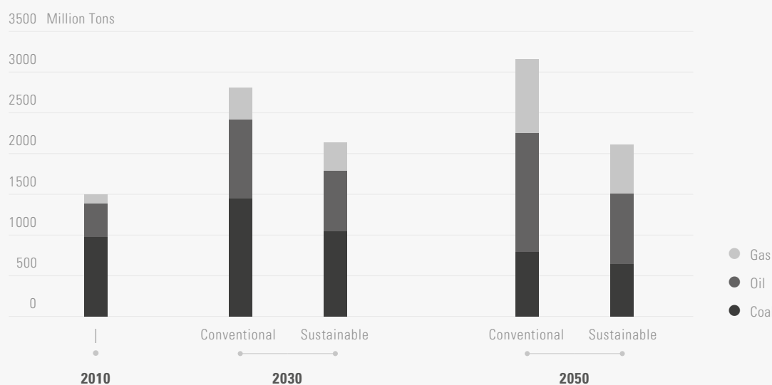
Figure 3.5: CO 2 Emissions
