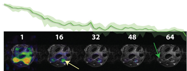
FIG. 2. A representative image series (image 1 - image 64) of a ^1\text{H} T_2 weighted FSE axial slice overlaid hyperpolarized [^{13}\text{C},^{15}\text{N}]\text{urea} with each image constructed by eight radial spokes. The images are normalized to the first image of the series (all images are shown logarithmic scaled) and the green line (solid) is the ROI time curve (transparent illustrates SD) from the renal cortex (green arrow). An intra-renal difference in signal is observable after 16 s (yellow arrow) showing elevated signal in the medulla, while no or little signal is observable after 512 refocusing pulses (image 64).
