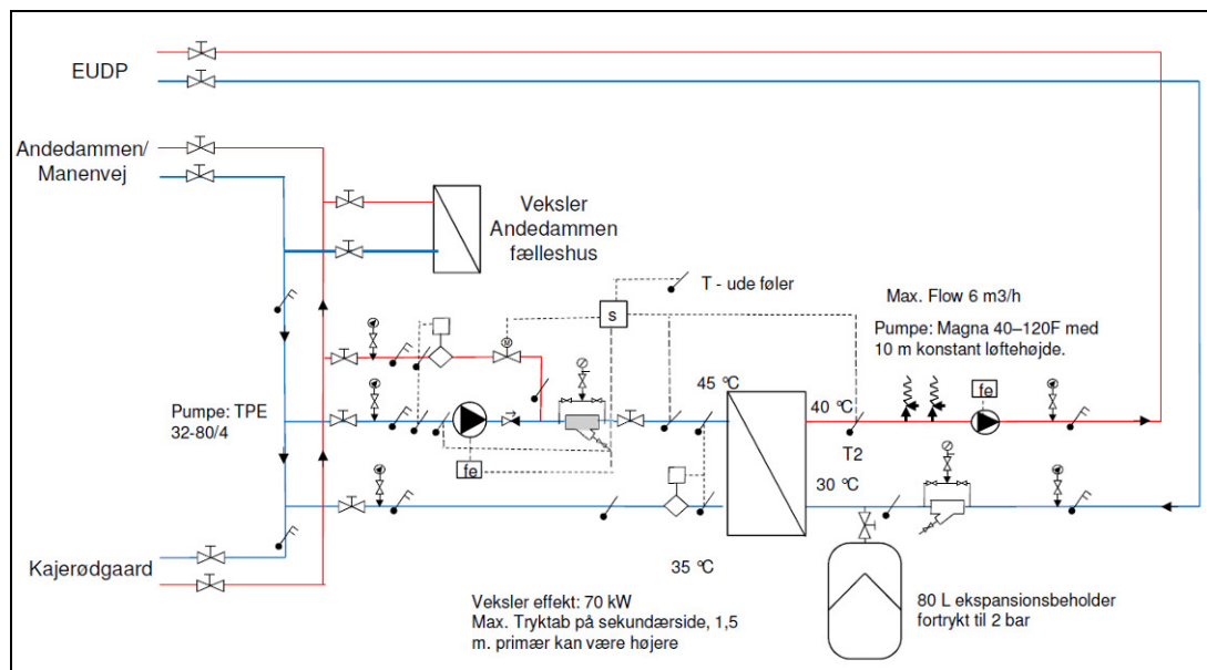
Figure 13: System for establishment of the low temperature supply system
