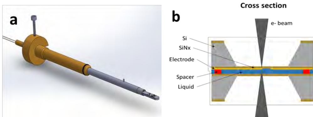
Figure 1. a). Schematic view of the manufactured TEM holder with liquid flow and 5 electrical contacts; b). Schematic cross section view of a double-chip setup with electron transparent window (SiNx) which is used for observing.
