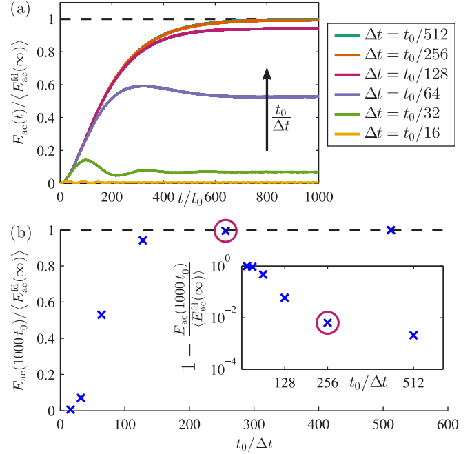
FIG. 2. (Color online) Numerical convergence and temporal resolution. (a) Graphs of the buildup of acoustic energy E_{\text{ac}}(t) in the time-domain simulations calculated with different fixed time steps \Delta t . The energy of the time-domain simulations is normalized with respect to the energy \langle E_{\text{ac}}^{\text{fd}}(\infty) \rangle of the steady solution in the frequency domain, and should thus converge towards unity. In all simulations the actuation frequency equals the resonance frequency discussed in Sec. IV A. (b) Acoustic energy E_{\text{ac}}(1000 t_0) at t = 1000 t_0 , normalized by \langle E_{\text{ac}}^{\text{fd}}(\infty) \rangle , and plotted versus the temporal resolution t_0/\Delta t of the oscillation. The inset is a semilog plot of the relative deviation of E_{\text{ac}}(1000 t_0) from \langle E_{\text{ac}}^{\text{fd}}(\infty) \rangle . The circled point in each graph indicates the time step \Delta t = t_0/256 used in all subsequent simulations.
