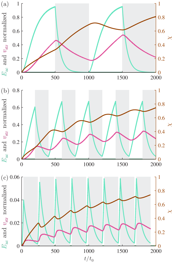
FIG. 8. (Color online) The same probes as in Fig. 7 but for the following pulsed actuation schemes: (a) actuation is on for 500 t_0 followed by no actuation for 500 t_0 repeatedly, (b) actuation is on for 200 t_0 followed by no actuation for 200 t_0 repeatedly, and (c) actuation is on for 30 t_0 followed by no actuation for 210 t_0 repeatedly.
