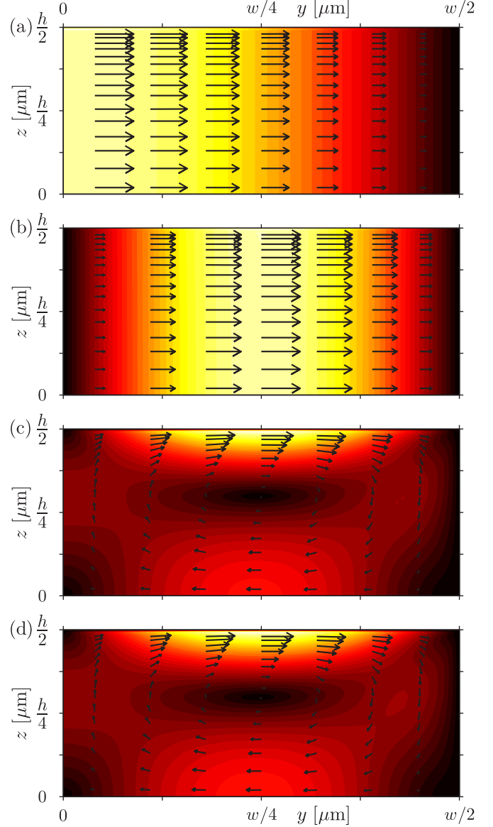
FIG. 4. (Color online) (a) Snapshot of the oscillatory first-order velocity field \mathbf{v}_1 (vectors) and its magnitude [color plot ranging from 0 m/s (black) to 0.7 m/s (white)] at t = 3000 t_0 . (b) Snapshot of the oscillatory second-order velocity field \mathbf{v}_2 (vectors) and its magnitude [color plot ranging from 0 m/s (black) to 0.02 m/s (white)] at t = 3000 t_0 . (c) Snapshot of the unsteady time-averaged second-order velocity field \langle \mathbf{v}_2 \rangle (vectors), Eq. (30), and its magnitude [color plot ranging from 0 mm/s (black) to 0.1 mm/s (white)] at t = 3000 t_0 . (d) Steady time-averaged second-order velocity field \langle \mathbf{v}_2^{\text{fd}}(\infty) \rangle (vectors), Eqs. (11) and (12), and its magnitude [color scaling as in (c)]. In both the time-domain and the frequency-domain simulations the parameters of the oscillating velocity boundary condition were \omega = 2\pi f_{\text{res}} and v_{bc} = \omega d , with wall displacement d = 1 nm.
