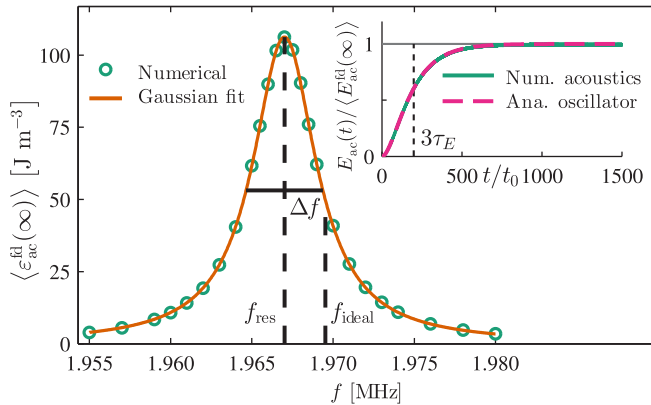
FIG. 3. (Color online) Resonance curve and buildup of acoustic energy. The numerical acoustic energy density \langle E_{ac}^{fd}(\infty) \rangle/V (circles) for different frequencies of the boundary actuation and a Gaussian fit (full line) to the numerical data. f_{res} = 1.9670094(7) MHz and \Delta f = 4.727(2) kHz are the fitted resonance frequency at the center of the peak and the line width, while f_{ideal} = c_s/(2w) is the frequency corresponding to matching a half wavelength with the channel width. The inset shows the numerical buildup of the acoustic energy (full line) for actuation at the resonance frequency, \omega = 2\pi f_{res} , along with the analytical prediction Eq. (23) (dashed line) for a single harmonic oscillator with the same resonance frequency and quality factor Q = f_{res}/\Delta f = 416 . The resonance relaxation time is \tau_E = Q/\omega = 66 t_0 .
