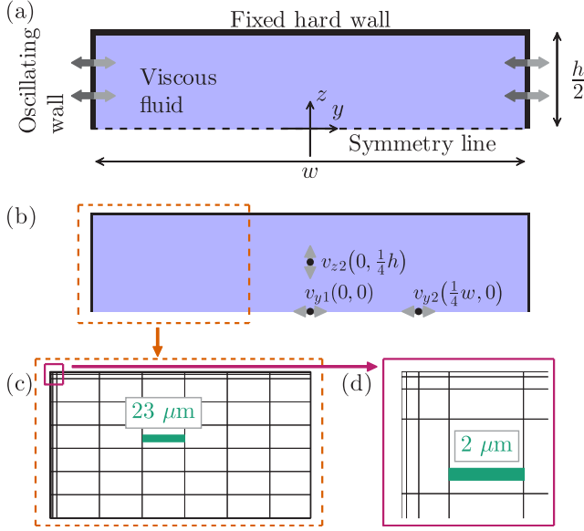
FIG. 1. (Color online) (a) Sketch of the rectangular computational domain in the yz plane representing the upper half of a rectangular cross section of a long straight microchannel of width w = 380 \mu\text{m} and height h = 160 \mu\text{m} as in Ref. [21]. The thick arrows indicate in-phase oscillating velocity actuation at the left and right boundaries. (b) The three black points indicate positions at which the velocity components (gray arrows), defined in Eq. (29) later in the paper, are probed. (c) Sketch of the spatial mesh used for the discretization of the physical fields. (d) A zoom-in on the mesh in the upper left corner.
