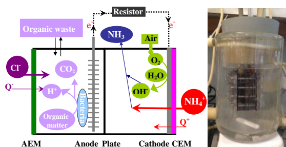
Figure 1 Schematic of the SMRC (A) and the image of the integrated SMRC-CSTR (B). \text{Q}^+ and \text{Q}^- are unspecified cations and anions, respectively.
