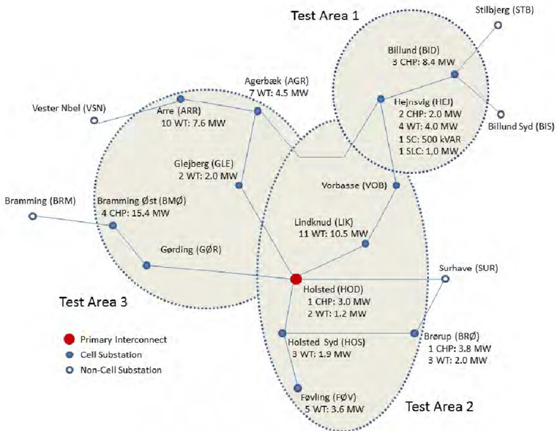
Figure 12-6 Topology of the Cell.
