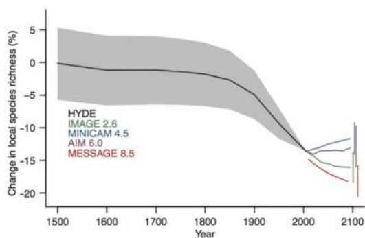
Projected net change in local species richness worldwide from 1500 to 2095; LBII additionally discounts species not in the original assemblage. Future projections are based on the four Representative Concentration Pathway scenarios 6 . Grey shading and error bars show 95% confidence intervals. (From Newbold et al. 2015 Nature 520:45-50.)
