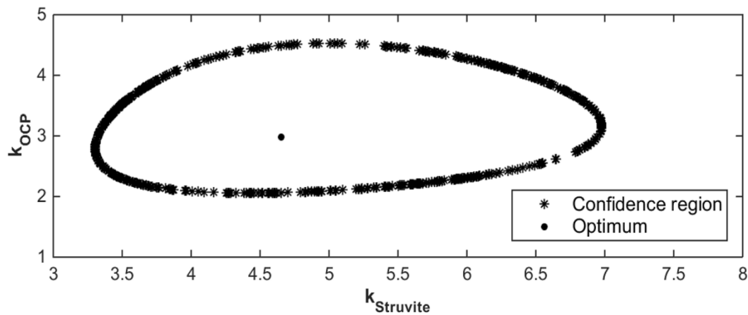
Fig. 2 – Confidence region at the 95% confidence limit for kinetic parameters determined from model fits of data from Aeration of ADS.
