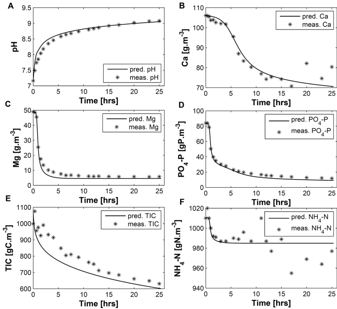
Fig. 1 – Representative experimental and modelling data for aeration tests on wastewater AD sludge (ADS) with struvite and calcium carbonate (monohydrate). The dotted and solid lines represent the experimental and simulation results of the batch precipitation experiment.
