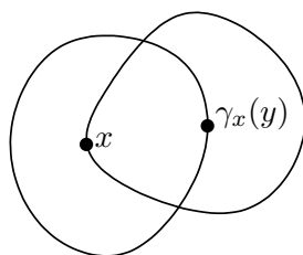
Figure 13: The necessary consistency condition for a field of unit spheres.
