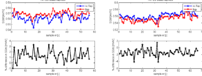
Fig. 11. Comparison of minimum flapwise bending moment at blade section root around tower passage between consecutive samples of no flap and flap activation (left: flap to max negative flap angle, right: flap to max positive flap deflection).
