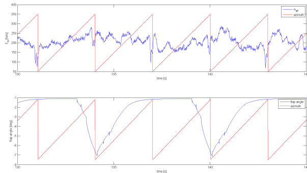
Fig. 9. Time series for flap azimuth control case at 5deg pitch with flap angle to P_{min} (max negative flap deflection) at tower passage (top to bottom: normal force, flap angle).
