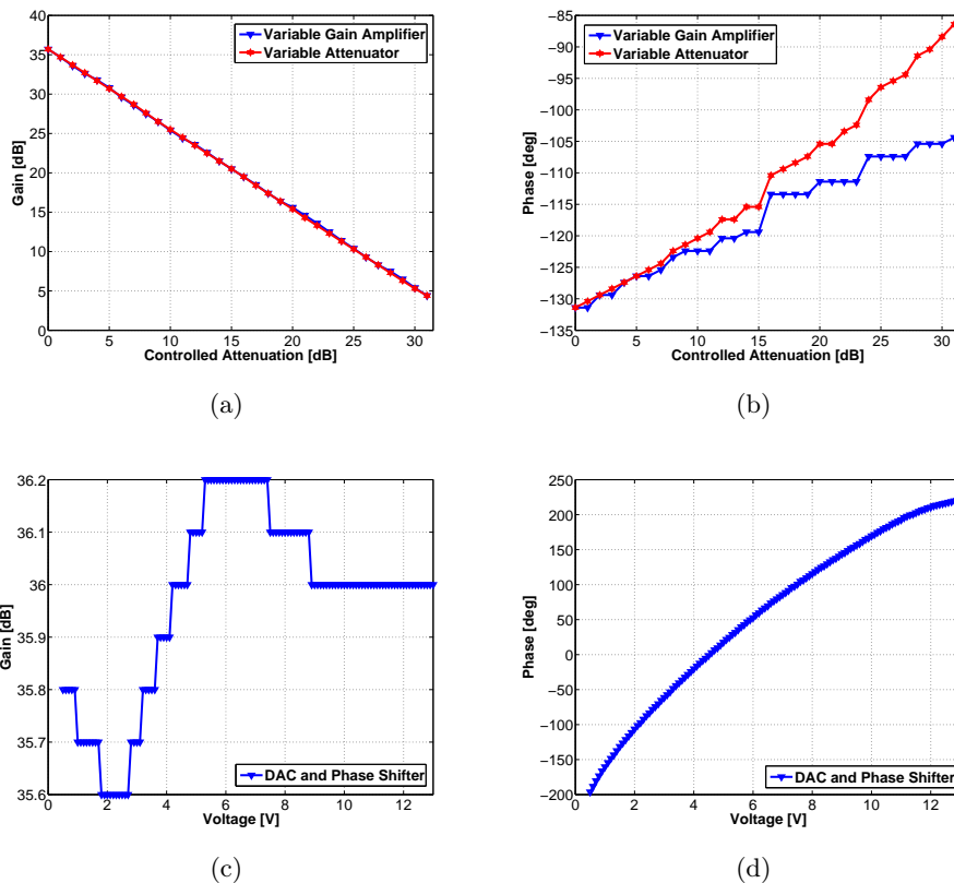
Figure 6.13: Gain and phase measurements of a transmitter. In (a) and (b), the DAC voltage was set to 1.5 V and the VA was set to 0 dB attenuation during VGA sweep and vice versa. In (c) and (d), the VA and VGA were both set to 0 dB attenuation while the DAC voltage was swept.
