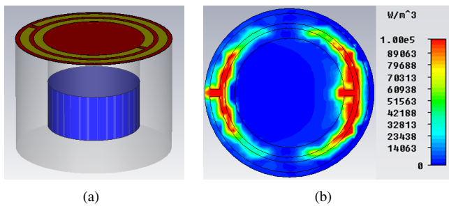
Fig. 3. In (a) a semi-transparent cylindrical capsule with the pharmaceutical drug inside and the split-ring resonators on top of a thin lid, on the capsule. In (b) the simulated power loss density in the lid is shown from the top.
