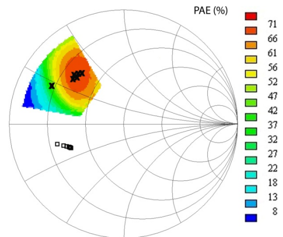
Fig. 5. Load pull data for a single transistor cell showing PAE circles at 9 GHz and synthesized impedances for each one of the 16 cells of a power bar, using the bondwire full wave model (crosses) and the inductor-based model (squares)
