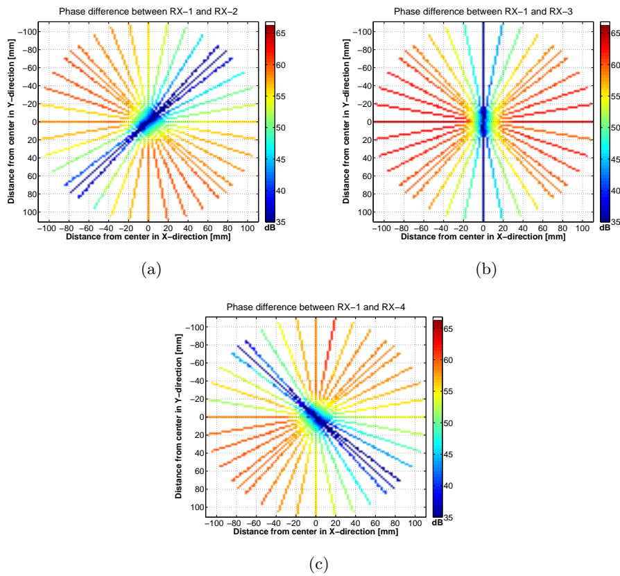
Figure D.8: Phase measurements in dBV scale as function of the internal antenna location inside the inner cylinder. (a) shows for the RX-2 - RX-1, (b) shows for the RX-3 - RX-1 and (c) shows for the RX-4 - RX-1
