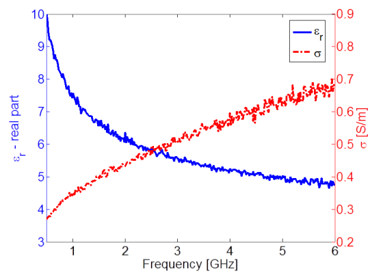
Figure B.1: Measured dielectric properties of glycerin.
