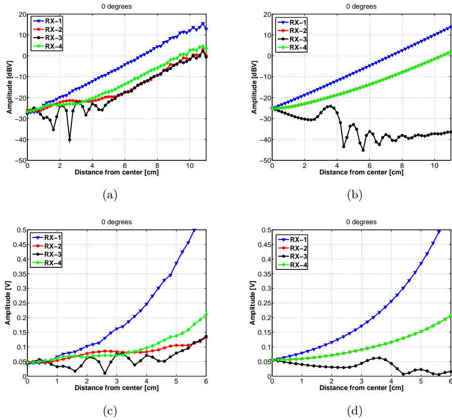
Figure 7.2: Amplitude measurements (left) and simulations (right) at 0^\circ . In (a) is measurement results in logarithmic scale, (b) simulation results in logarithmic scale, (c) measurement results while zoomed-in to the lower part in linear range and (d) simulation results while zoomed-in to the lower part in linear range.
