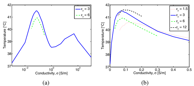
Fig. 4. Maximum temperature as a function of conductivity for various relative permittivities of the lid of a pharmaceutical drug capsule. Fig. (a) shows a wide range of conductivities while (b) shows narrow range.
