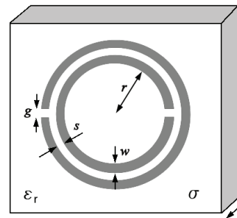
Fig. 2. A split-ring resonator with dimensional variables.
