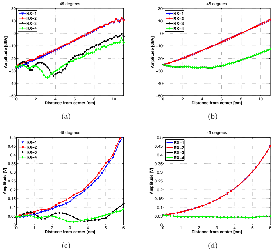
Figure 7.6: Amplitude measurements (left) and simulations (right) at 45^\circ . In (a) are measurement results in logarithmic scale, (b) simulation results in logarithmic scale, (c) measurement results while zoomed-in to the lower part in linear range and (d) simulation results while zoomed-in to the lower part in linear range.
