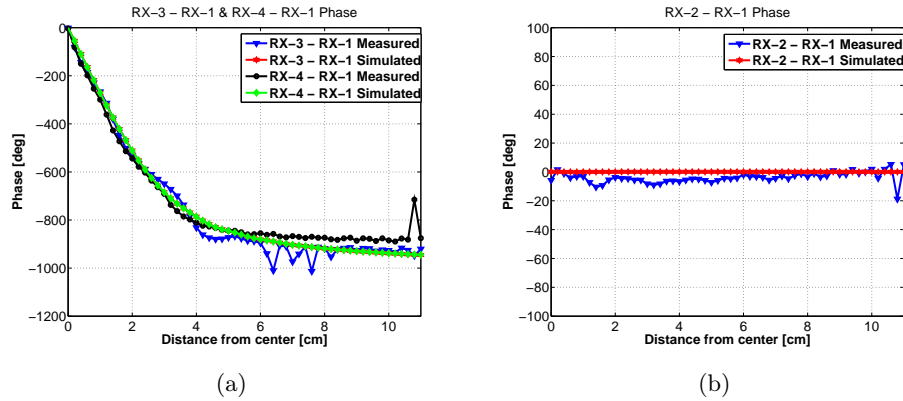
Figure 7.8: Phase measurement and simulation in COMSOL at 45^\circ . In (a) is the results for RX-3 - RX-1 and RX-4 - RX-1 and in (b) is the results for RX-2 - RX-1. The phase for RX-3 - RX-1 (red) is not easily seen for the simulation as it lies behind the green curve.
