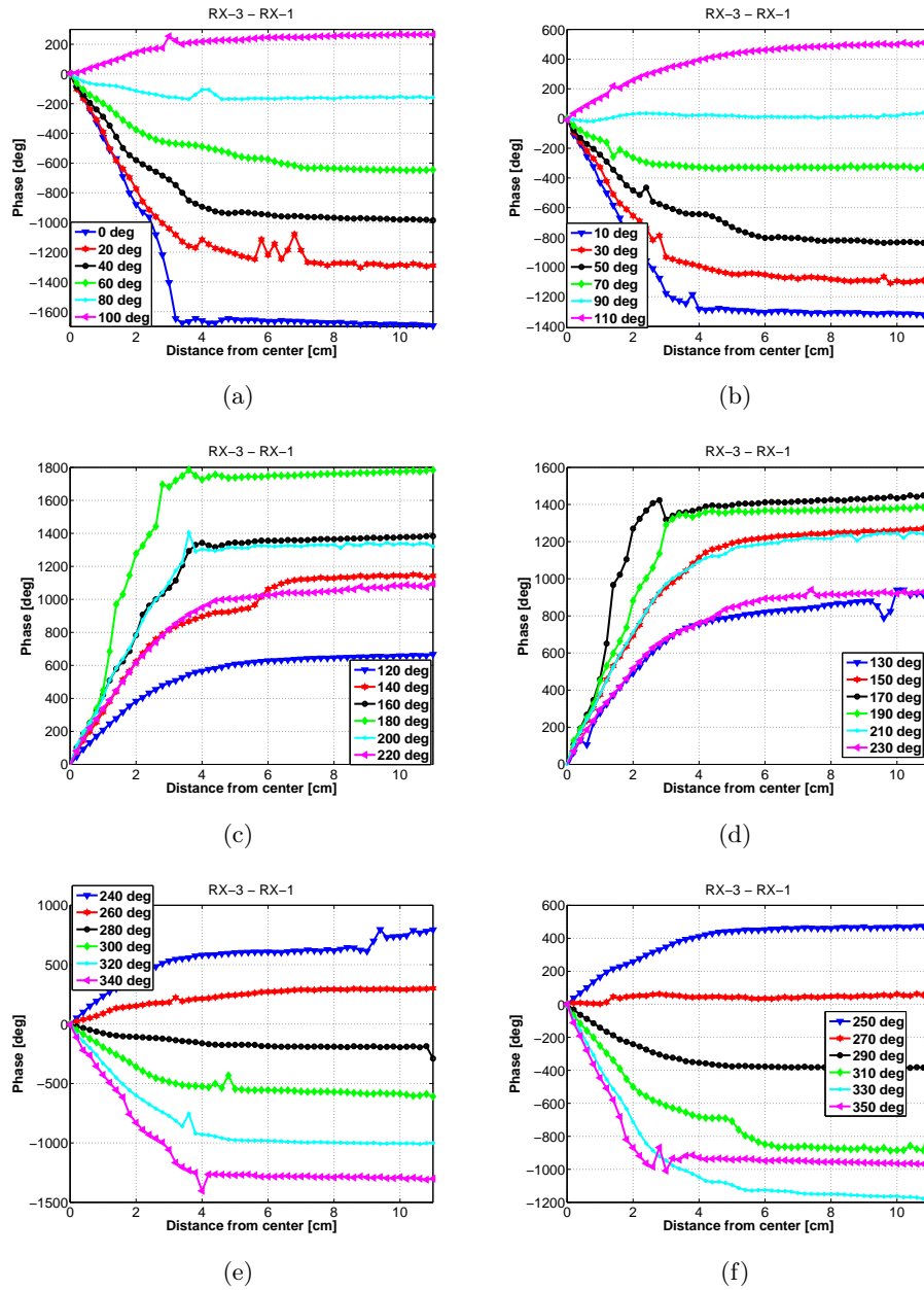
Figure D.5: Phase measurements of RX-3 - RX-1 for every 10 degree step. In (a), (c) and (e) are 0, 20, 40, 60 degrees etc. In (b), (d) and (f) are 10, 30, 50, 70 degrees etc.
