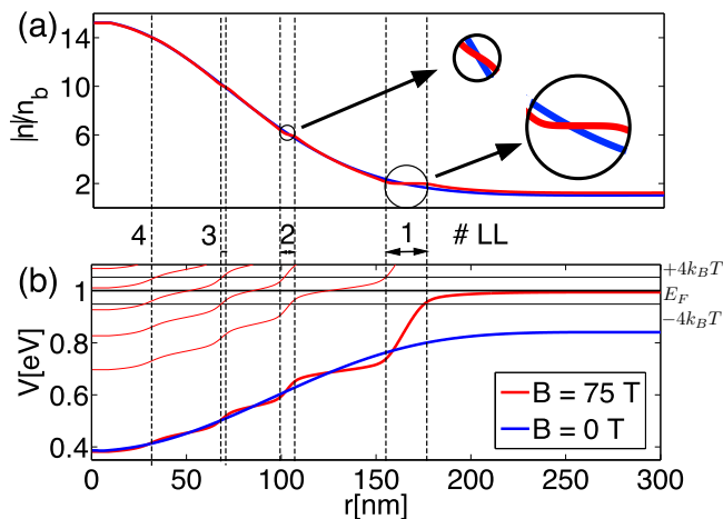
FIG. 2. (Color online) (a) Electrons density n vs distance r ; n is given in units of n_b = \frac{1}{2\pi l_B^2} , the number of states in each Landau level (LL) per unit area. Note that g = 2 for the zeroth LL and g = 4 otherwise; (b) potential profiles: the total self-consistent screened potential V(r) and the model potential V_{\text{mod}}(r) (bold red and blue lines, respectively). Parameters of the external potential V_{\text{ext}} : V_0 = 10 V, l_0 = 75 nm. E_F = eV_g = 1 eV (a window E_F \pm 4k_B T around E_F is indicated). Magnetic field B = 75 T. Thin red lines show V(r) + \hbar\omega_C\sqrt{n} with n = 1, 2, 3, 4 , and 5. The number of occupied Landau levels (#LL) is indicated in the figure.
