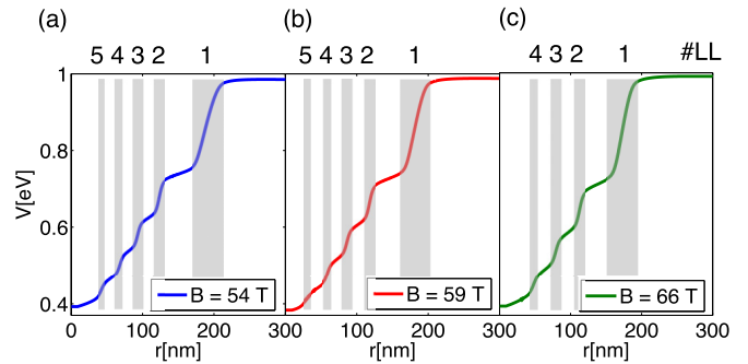
FIG. 3. (Color online) Potential profiles with a maximum of five Landau levels occupied for (a) B = 54 T and (b) B = 59 T, and with maximally four Landau levels occupied for (c) B = 66 T. Calculated from V_{\text{ext}} with V_0 = 10 V, l_0 = 75 nm, and eV_g = 1 eV. Regions with fully occupied Landau levels (incompressible strips) are indicated by gray strips and the number of occupied Landau levels.
