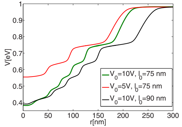
FIG. 6. (Color online) (a) Potential profiles for fixed magnetic field B = 50 T, gate voltage eV_g = 1 eV, and different dot parameters.
