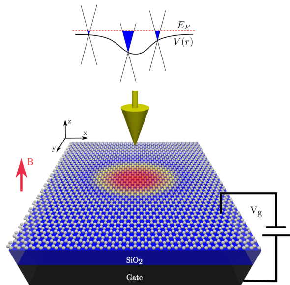
FIG. 1. (Color online) Sketch of a system under consideration representing a graphene sheet on an insulating substrate \text{SiO}_2 (blue) and a back gate (black). A quantum dot is created via an application of electrostatic potential (red) from a tip and a perpendicular magnetic field B . A gate voltage V_g is applied to the back gate. In the sketch of the profile of the quantum dot [V(r)] and the Fermi energy ( E_F ), we illustrate the Thomas-Fermi approximation, where the position of the Dirac point depends on r , and the density of states is calculated locally.
