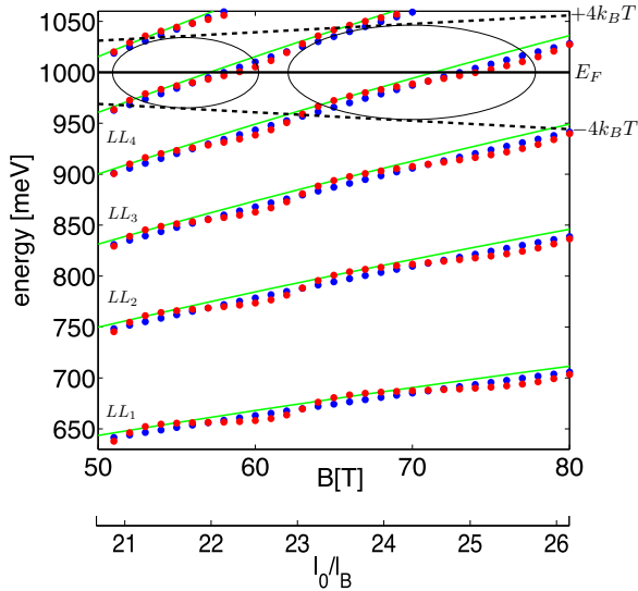
FIG. 4. (Color online) Eigenenergies vs magnetic field. Calculations are done for the total screened potential V(r) (blue dots) and for the model potential V_{\text{mod}}(r) with the Fermi energy E_F = eV_g = 1 eV. Green lines indicate pure Landau levels LL_n with the energies E_n = \hbar\omega_C\sqrt{n} + U_0 ; U_0 = 386.99 meV. Ellipses indicate plateaus formed due to the pinning of the eigenstates belonging to the partially filled states to the Fermi energy. The window E_F \pm 4k_B T corresponding to the states that are partially filled is indicated. Note that a temperature T introduced to achieve a convergence of numerical calculations increases with B . The magnetic field is indicated both in units of T and as a ratio l_0/l_B .
