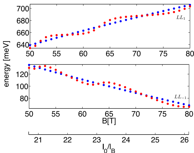
FIG. 5. (Color online) The same as in Fig. 4 but showing the eigenstates corresponding to LL_1 and LL_{-1} .
