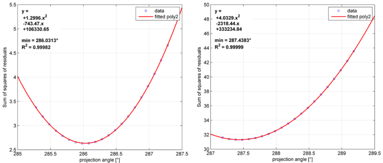
Figure 16. LOS direction evaluation using the RSS process: 5-beam (left, LOSO) and ZDM (right) lidars
