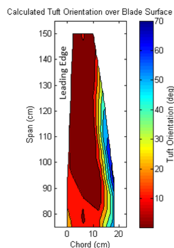
Fig. 3 Average tuft orientation at \lambda = 6.3 .
