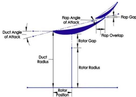
Fig. 2 DWT Geometry
