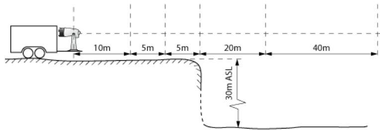
Fig. 2 Vertical wind profile measurement locations with respect to LiDAR and cliff edge.
