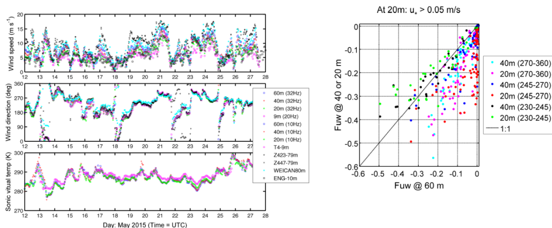
Fig. 2 Left: Hourly average mean wind speed, direction and temperature from the different instruments during the field experiment. Right: Profile of momentum flux at the 80 MM (400-m from the coast) conditionally sampled by wind direction. Note the presence of inverted flux profiles for flow along the cliff.
